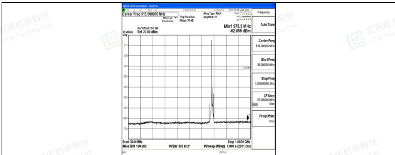
Band71_10MHz_16QAM_133422_1RB#0_30~1000_30~1000
