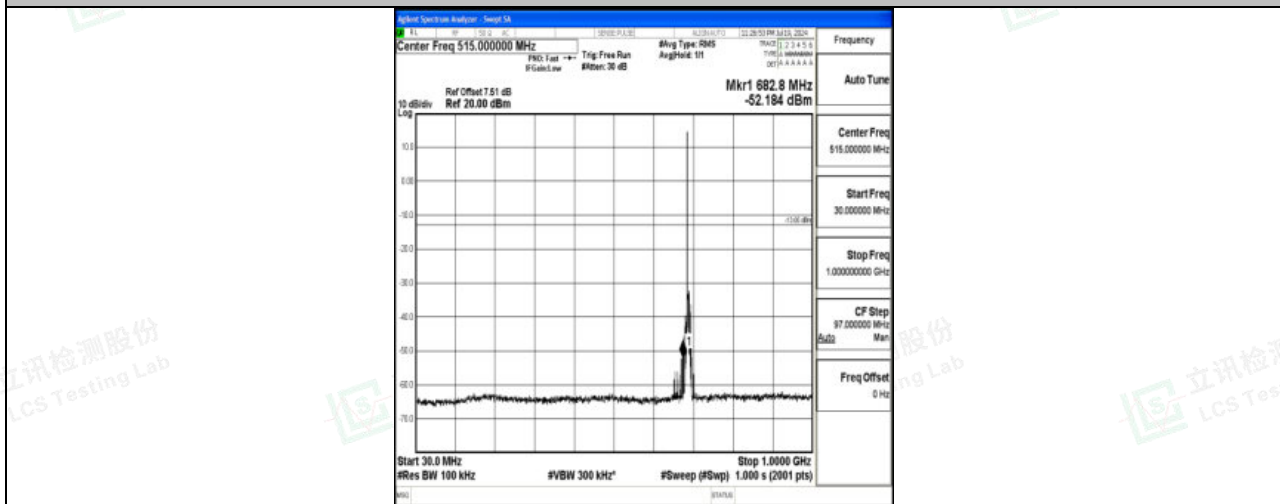
Band71_5MHz_16QAM_133447_1RB#0_30~1000_30~1000
