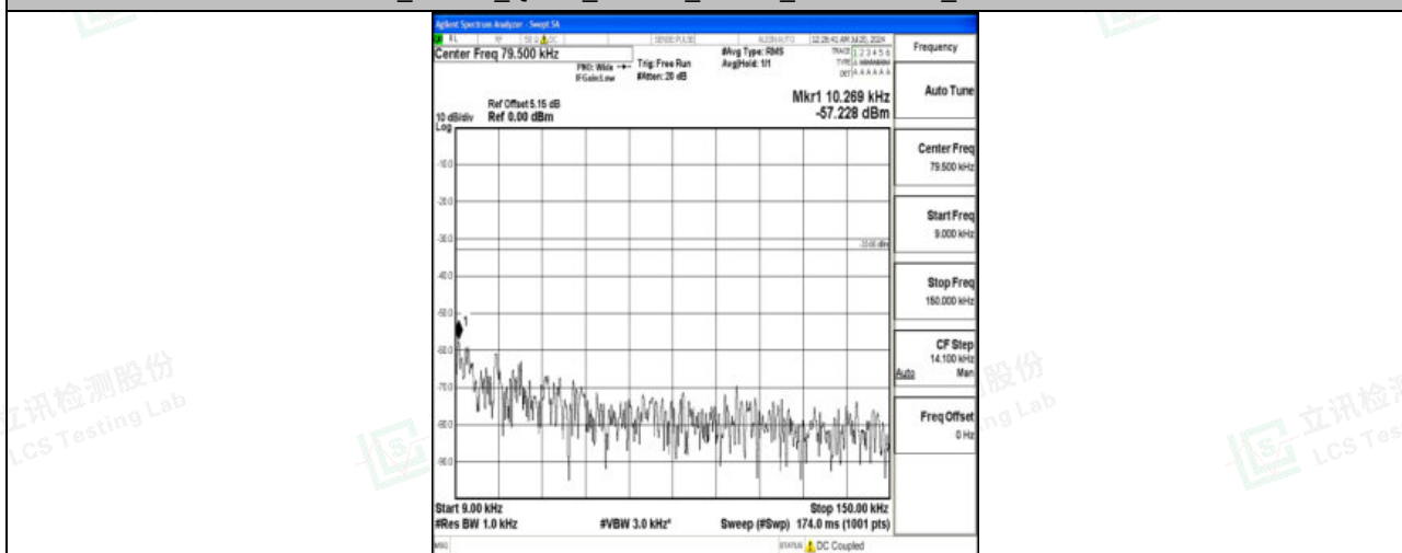
Band71_15MHz_16QAM_133397_1RB#0_0.009~0.15_0.009~0.15
