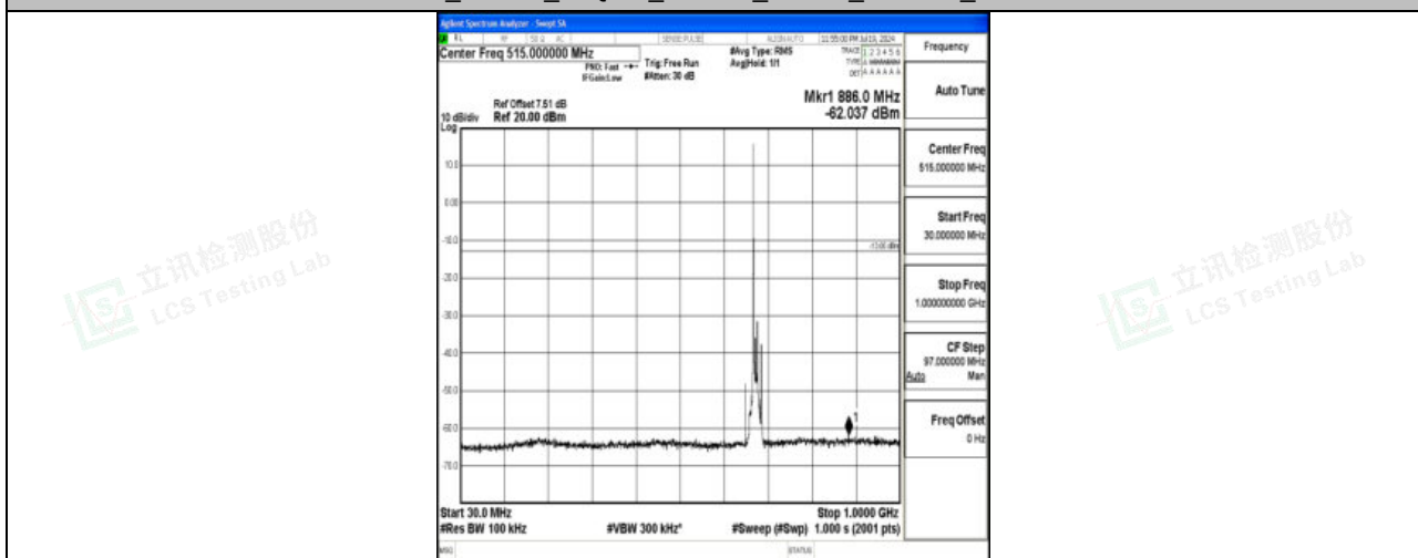
Band71_10MHz_16QAM_133297_1RB#0_30~1000_30~1000
