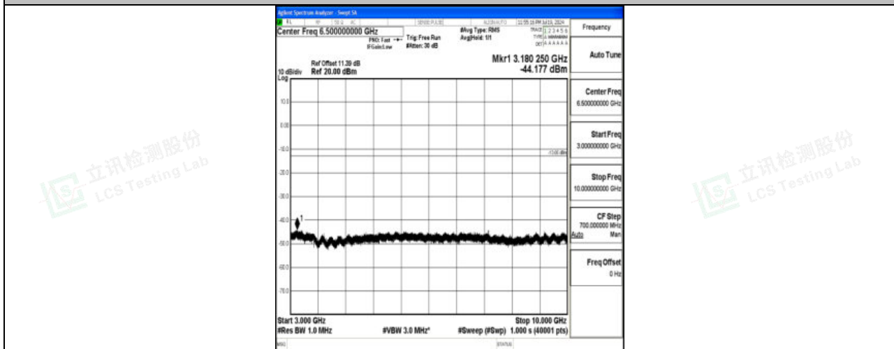
Band71_10MHz_16QAM_133297_1RB#0_3000~10000_3000~10000
