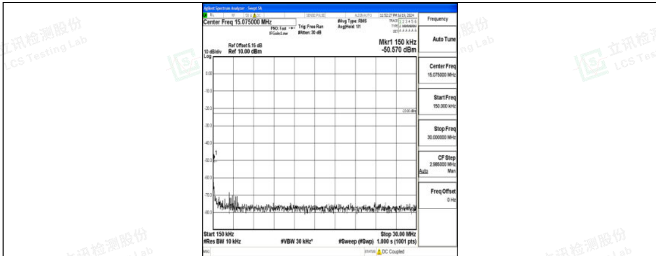
Band71_10MHz_16QAM_133172_1RB#0_0.15~30_0.15~30
