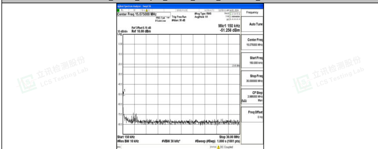
Band71_20MHz_16QAM_133322_1RB#0_0.15~30_0.15~30
