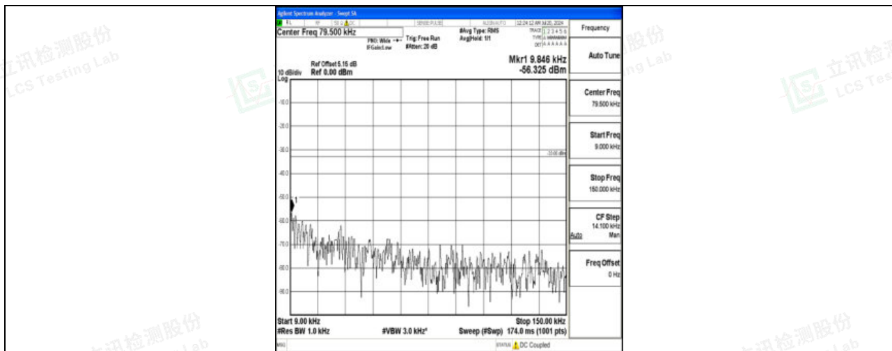
Band71_15MHz_16QAM_133297_1RB#0_0.009~0.15_0.009~0.15
