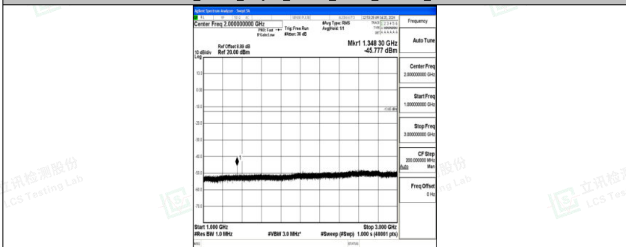
Band71_20MHz_16QAM_133322_1RB#0_1000~3000_1000~3000
