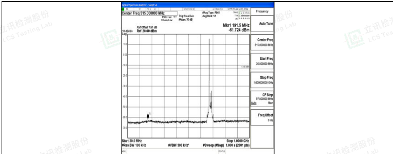
Band71_20MHz_16QAM_133372_1RB#0_30~1000_30~1000
