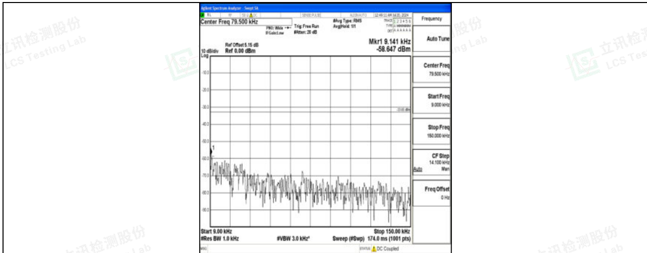
Band71_20MHz_QPSK_133222_1RB#0_0.009~0.15_0.009~0.15
