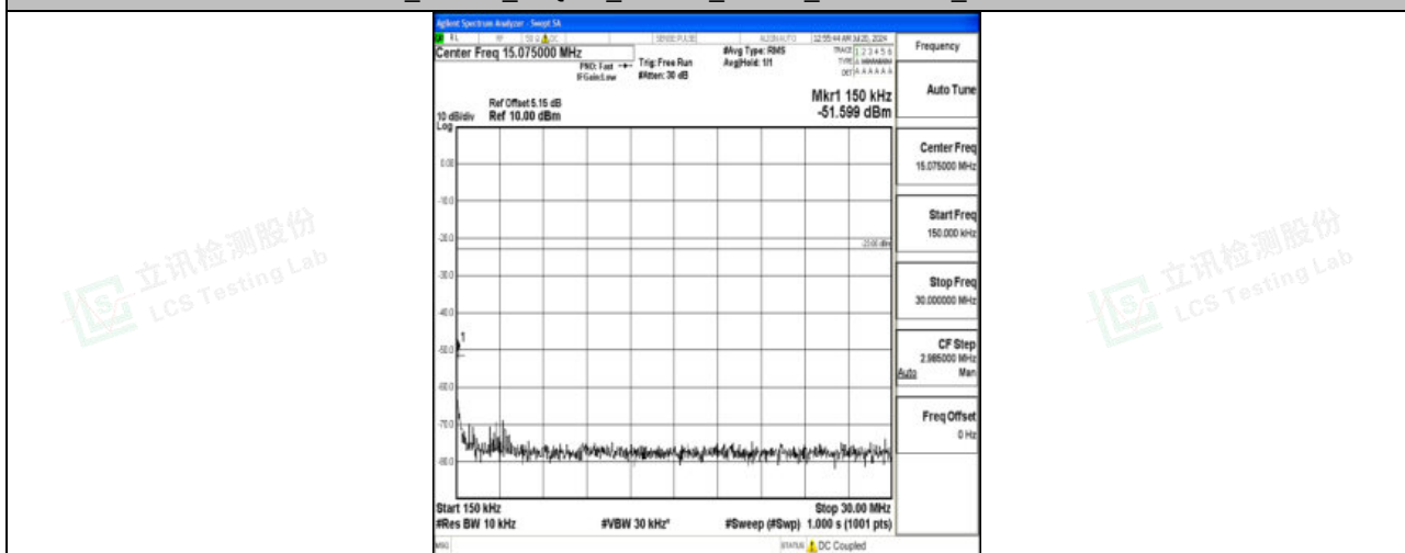
Band71_20MHz_16QAM_133372_1RB#0_0.15~30_0.15~30
