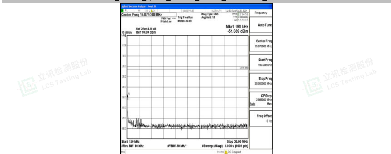
Band71_20MHz_QPSK_133322_1RB#0_0.15~30_0.15~30
