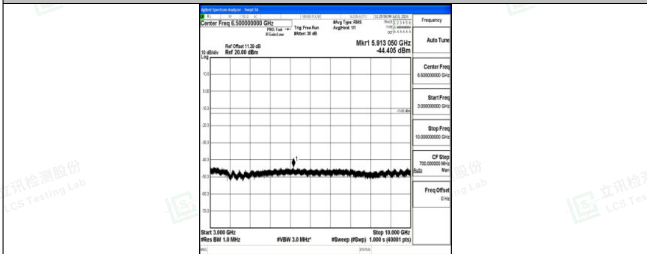
Band71_5MHz_QPSK_133447_1RB#0_3000~10000_3000~10000
