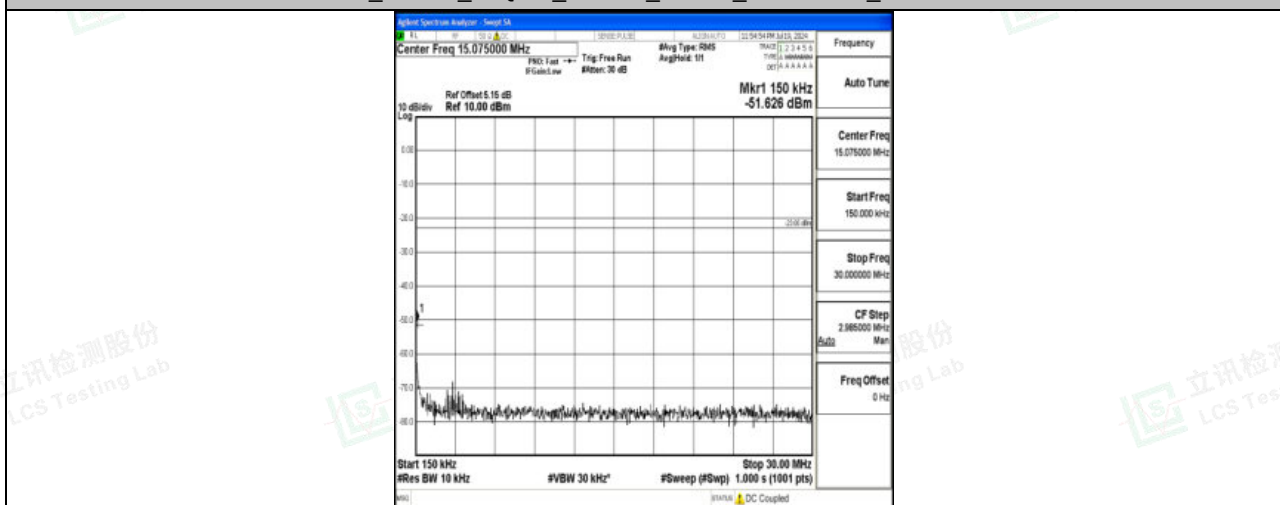
Band71_10MHz_16QAM_133297_1RB#0_0.15~30_0.15~30
