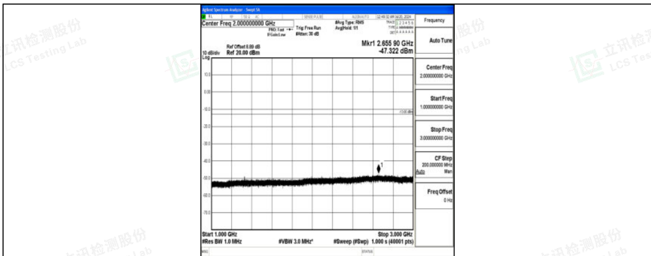
Band71_20MHz_QPSK_133222_1RB#0_1000~3000_1000~3000
