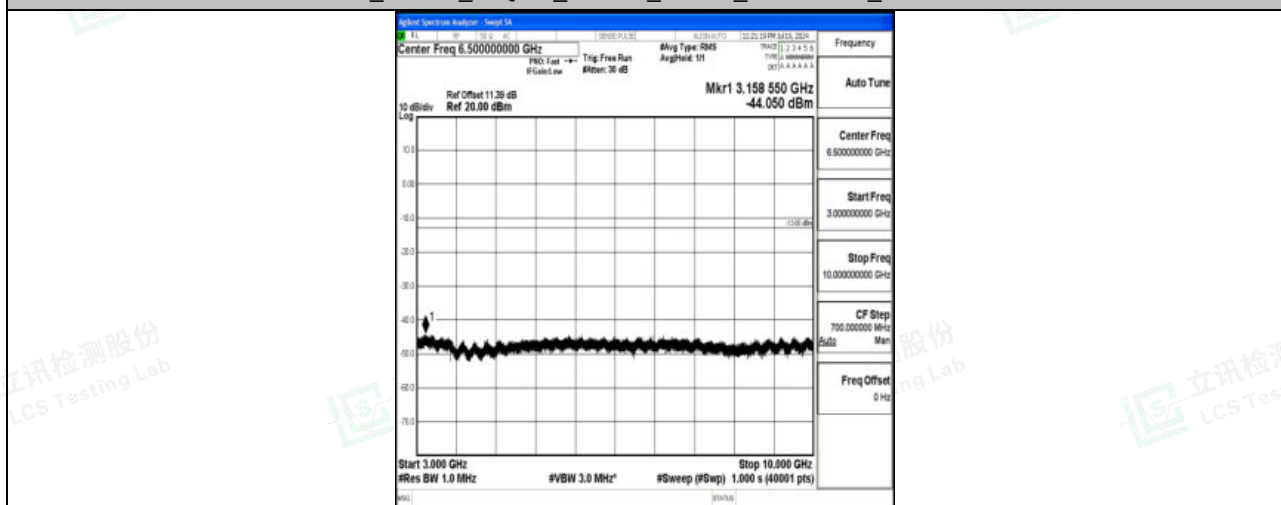
Band71_5MHz_QPSK_133147_1RB#0_3000~10000_3000~10000
