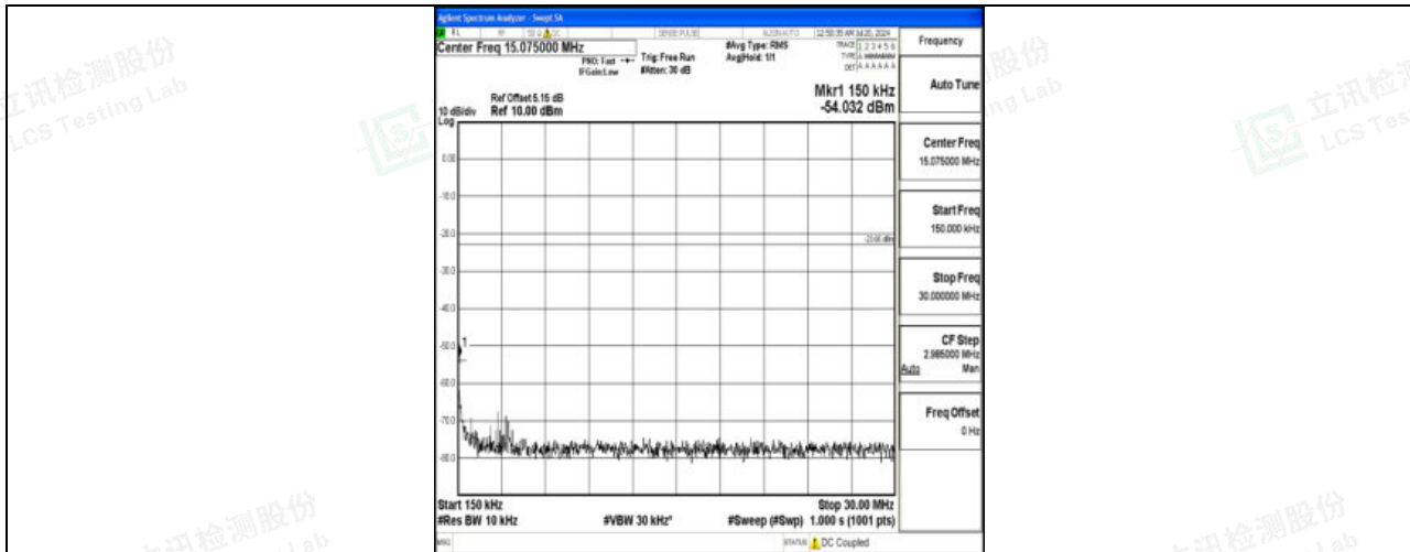
Band71_20MHz_16QAM_133222_1RB#0_0.15~30_0.15~30
