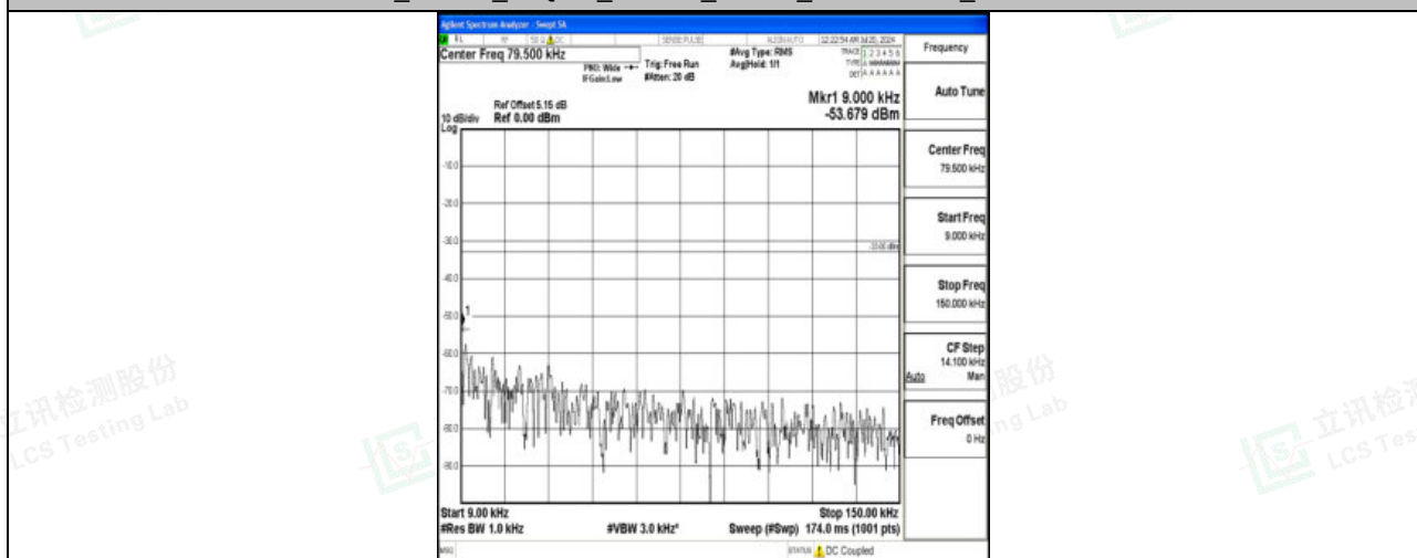
Band71_15MHz_QPSK_133297_1RB#0_0.009~0.15_0.009~0.15
