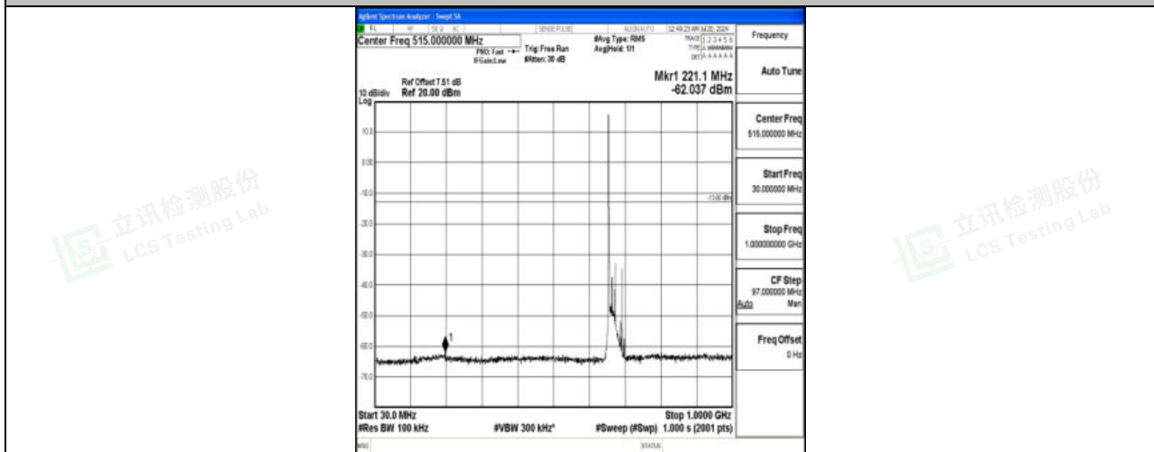
Band71_20MHz_QPSK_133222_1RB#0_30~1000_30~1000
