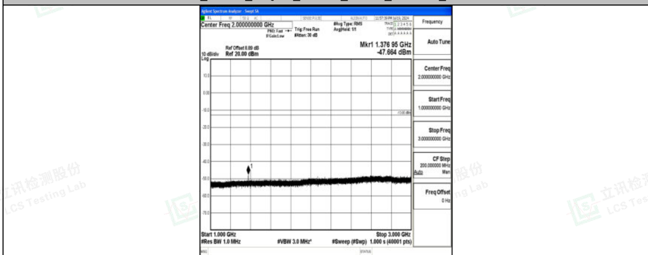
Band71_10MHz_16QAM_133422_1RB#0_1000~3000_1000~3000
