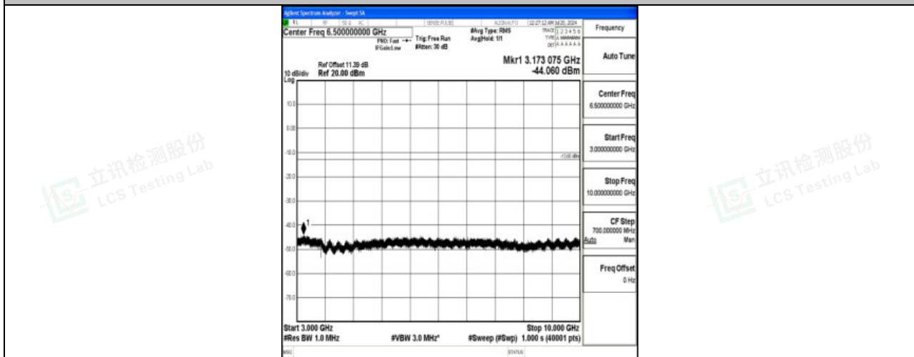
Band71_15MHz_16QAM_133397_1RB#0_3000~10000_3000~10000
