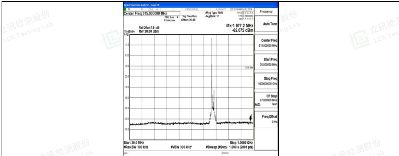
Band71_20MHz_QPSK_133322_1RB#0_30~1000_30~1000
