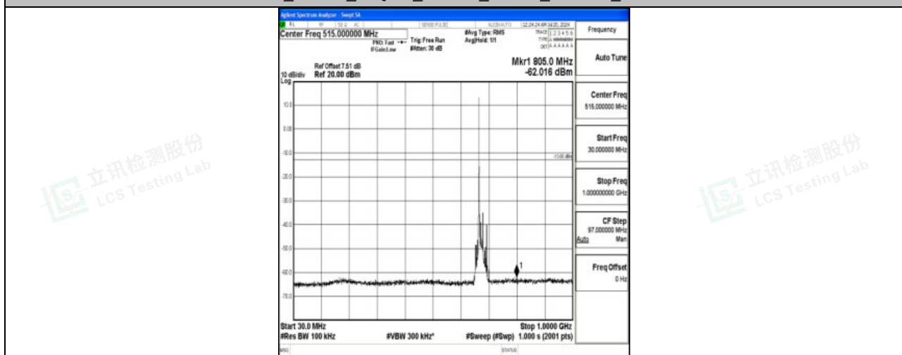
Band71_15MHz_16QAM_133297_1RB#0_30~1000_30~1000
