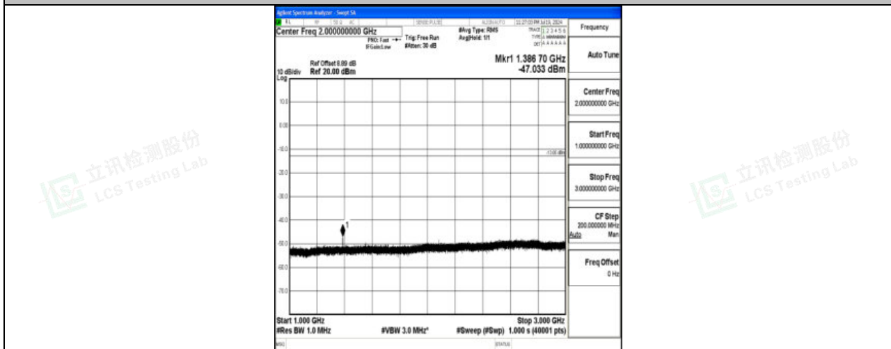
Band71_5MHz_16QAM_133447_1RB#0_1000~3000_1000~3000
