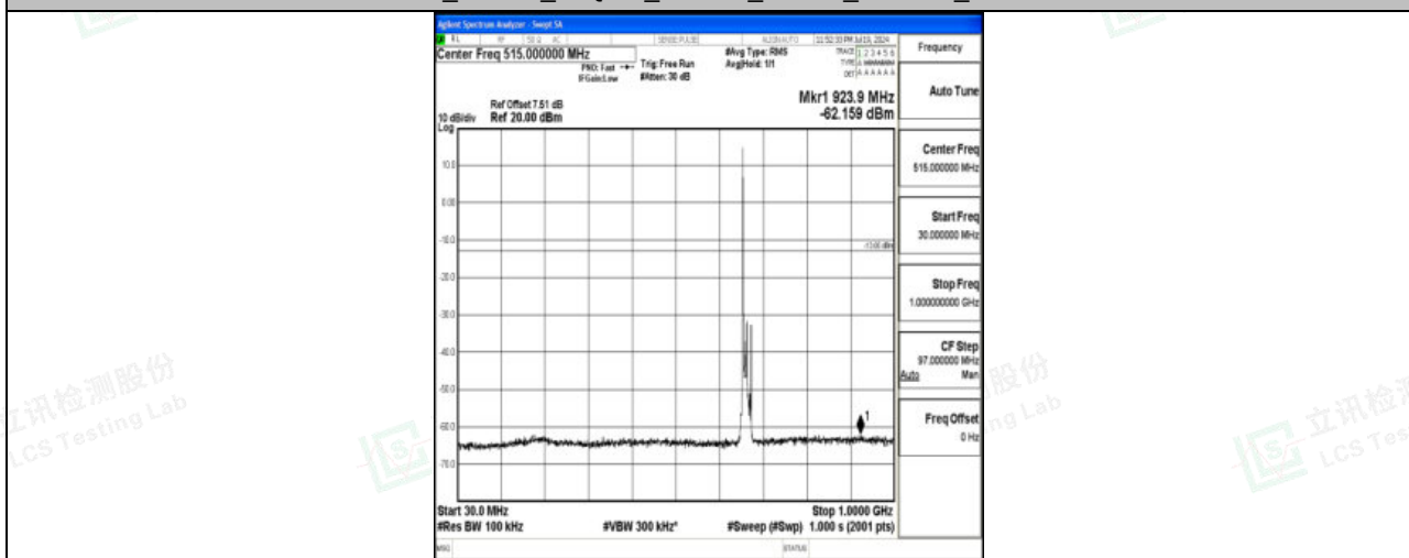
Band71_10MHz_16QAM_133172_1RB#0_30~1000_30~1000
