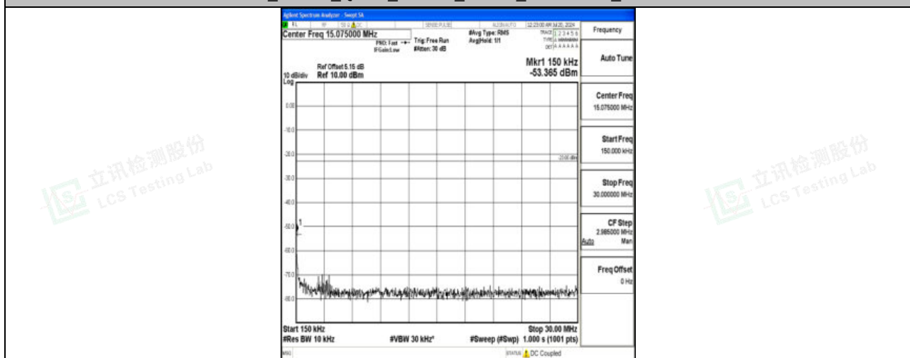
Band71_15MHz_QPSK_133297_1RB#0_0.15~30_0.15~30
