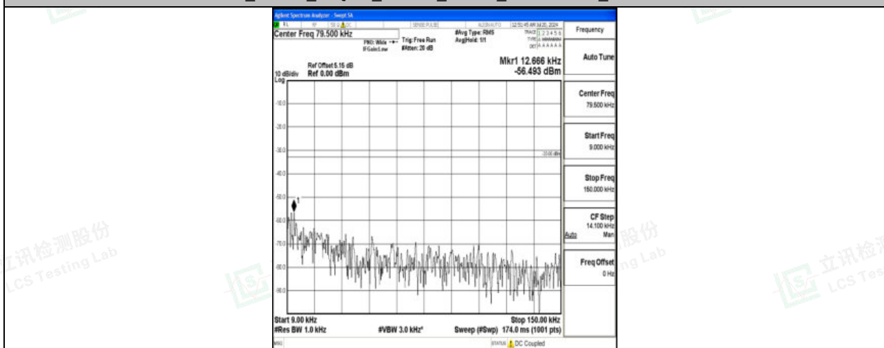
Band71_20MHz_QPSK_133322_1RB#0_0.009~0.15_0.009~0.15
