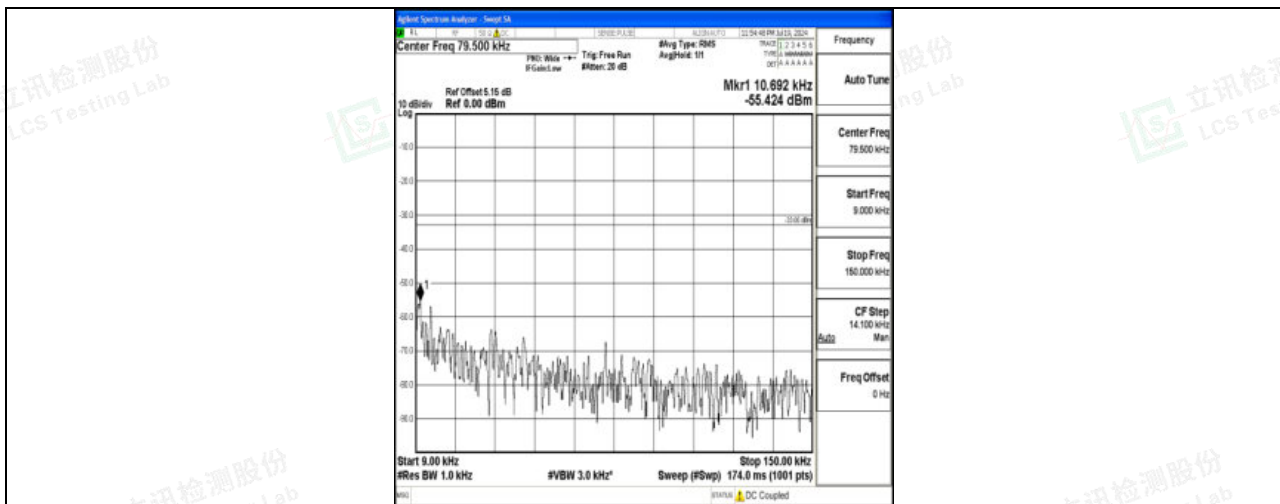
Band71_10MHz_16QAM_133297_1RB#0_0.009~0.15_0.009~0.15
