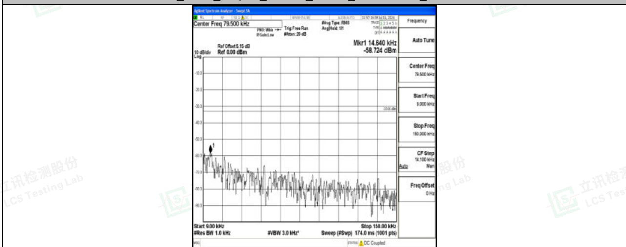
Band71_10MHz_16QAM_133422_1RB#0_0.009~0.15_0.009~0.15
