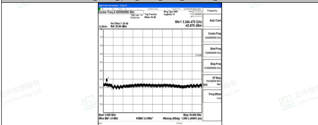
Band71_20MHz_QPSK_133222_1RB#0_3000~10000_3000~10000
