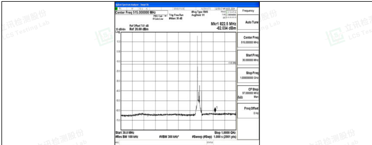
Band71_20MHz_16QAM_133322_1RB#0_30~1000_30~1000
