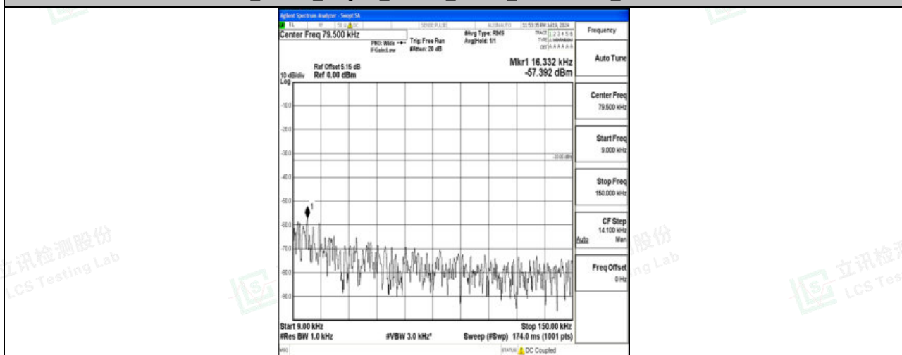
Band71_10MHz_QPSK_133297_1RB#0_0.009~0.15_0.009~0.15
