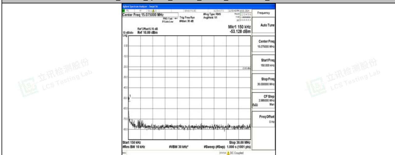
Band71_10MHz_QPSK_133297_1RB#0_0.15~30_0.15~30
