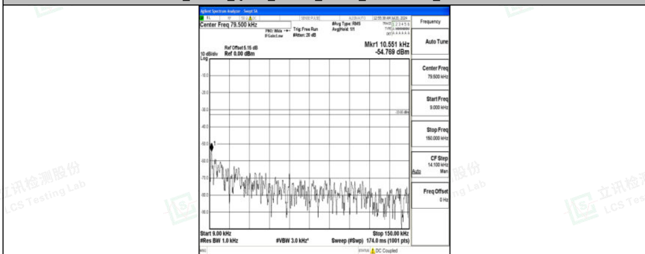
Band71_20MHz_16QAM_133372_1RB#0_0.009~0.15_0.009~0.15
