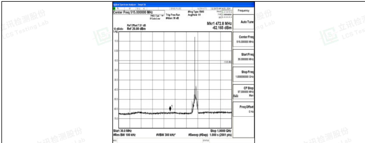
Band71_15MHz_16QAM_133397_1RB#0_30~1000_30~1000
