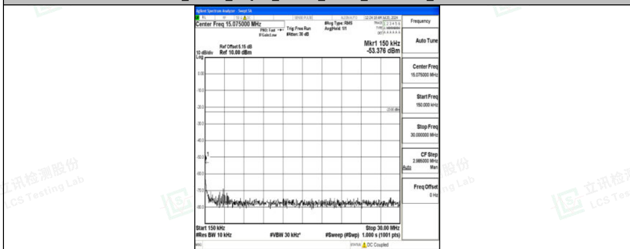
Band71_15MHz_16QAM_133297_1RB#0_0.15~30_0.15~30
