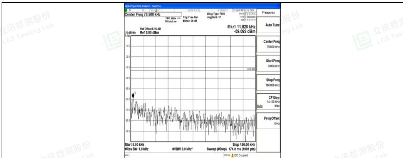
Band71_10MHz_QPSK_133422_1RB#0_0.009~0.15_0.009~0.15
