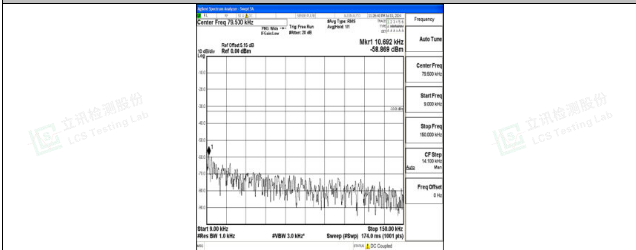
Band71_5MHz_16QAM_133447_1RB#0_0.009~0.15_0.009~0.15
