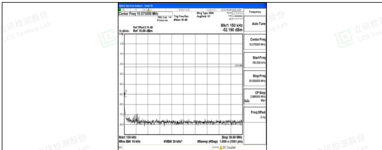
Band71_15MHz_16QAM_133197_1RB#0_0.15~30_0.15~30
