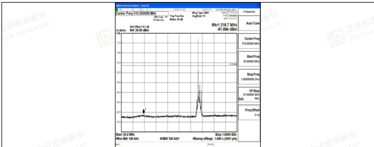
Band71_15MHz_QPSK_133297_1RB#0_30~1000_30~1000
