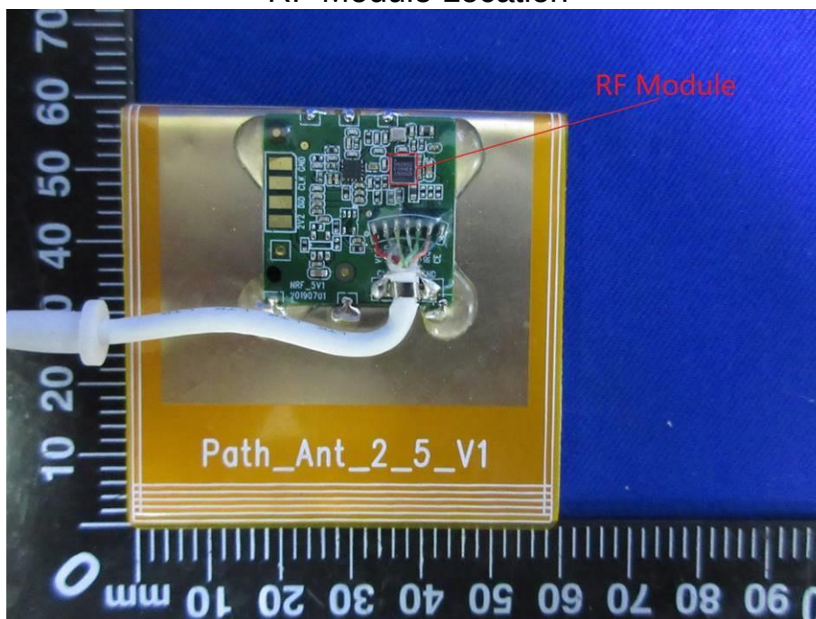
RF Module Location
