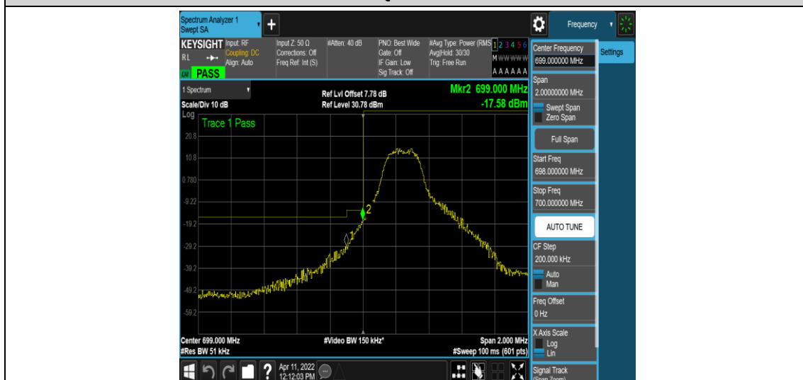
Band12-3MHz-16QAM-23025-1RB#0
