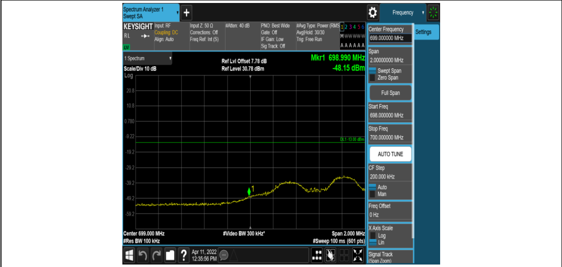
Band12-5MHz-QPSK-23035-1RB#24
