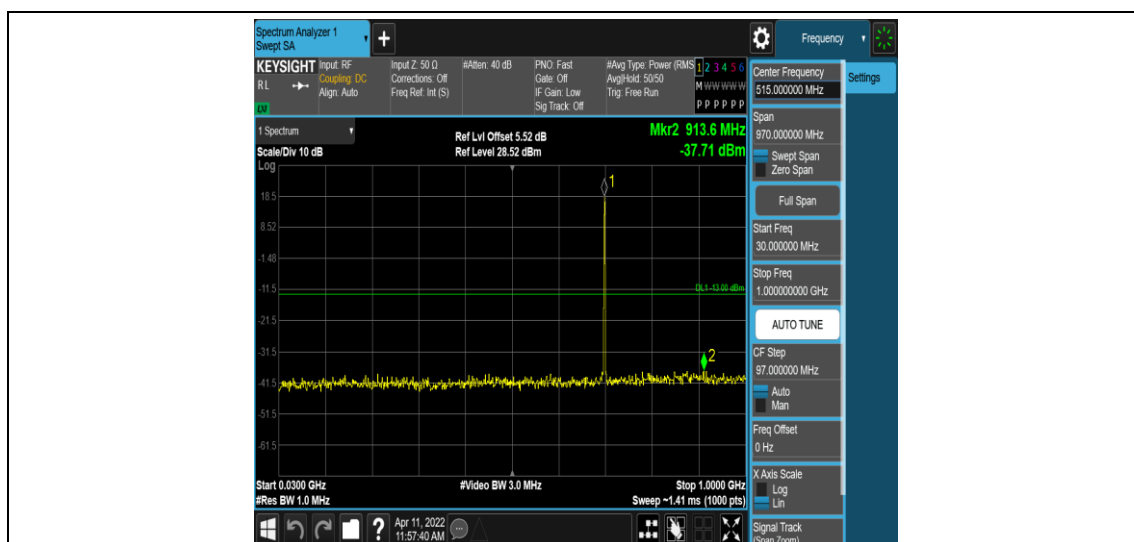
Band12-1.4MHz-16QAM-23095-1RB#0-Range3:30~1000MHz
