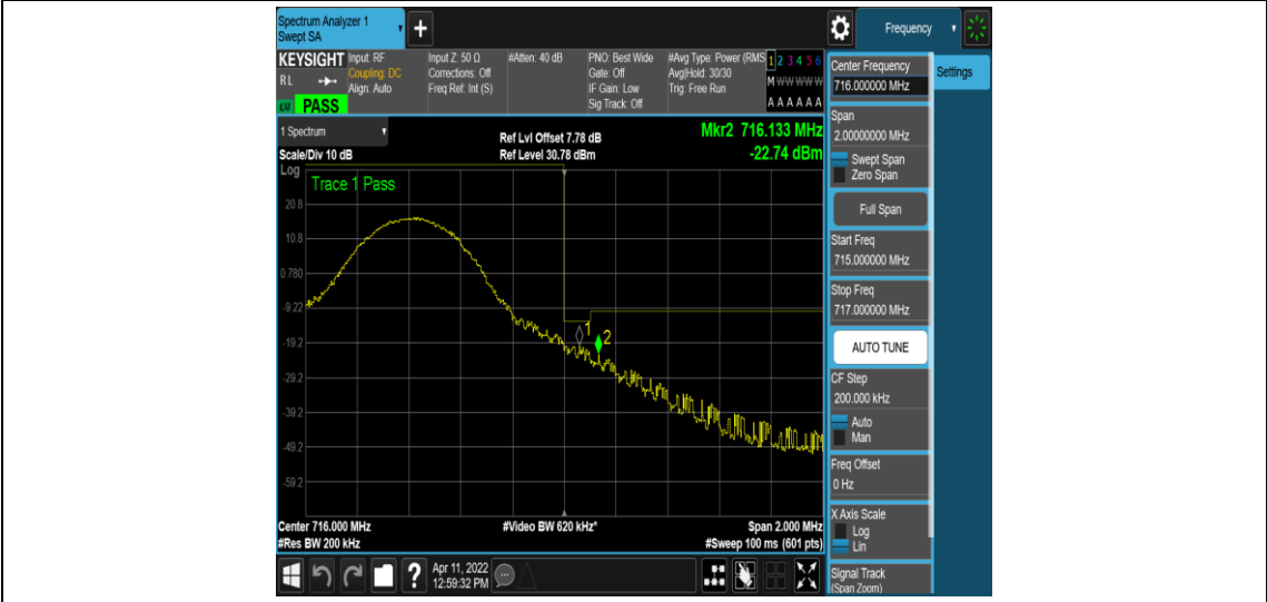
Band12-10MHz-16QAM-23130-1RB#49
