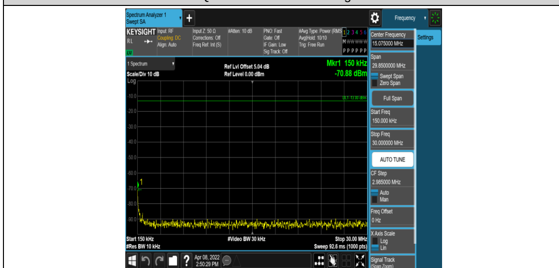
Band2-3MHz-16QAM-18900-1RB#0-Range2:0.15~30MHz
