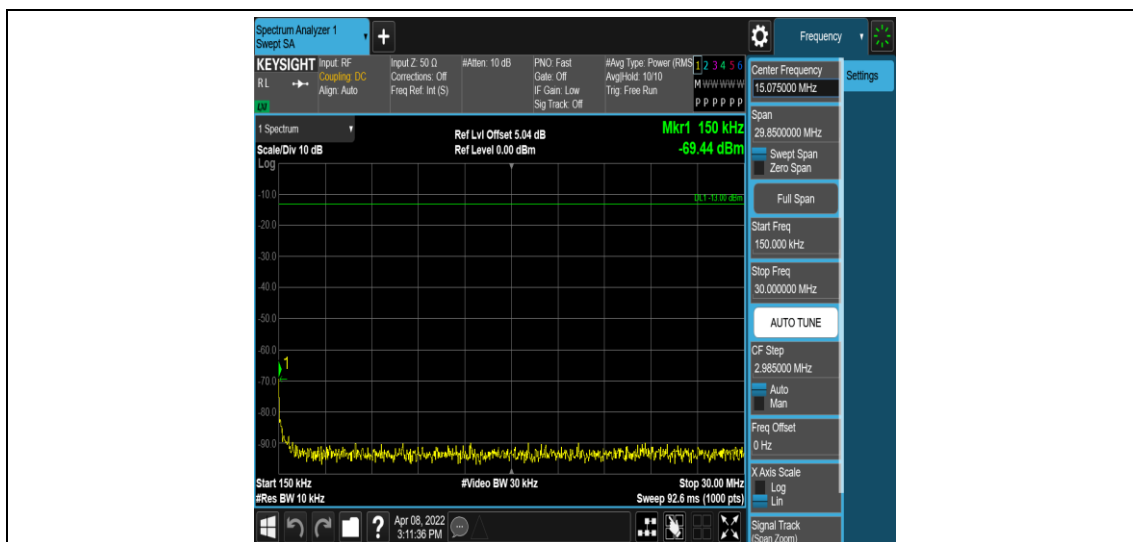
Band2-5MHz-16QAM-18625-1RB#0-Range2:0.15~30MHz
