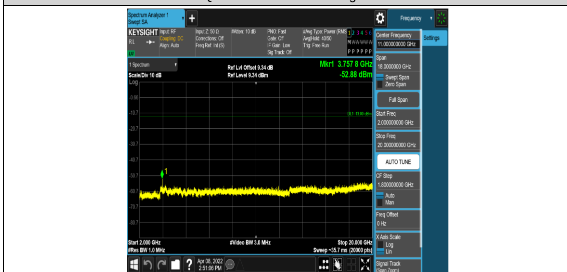
Band2-3MHz-16QAM-18900-1RB#0-Range5:2000~20000MHz
