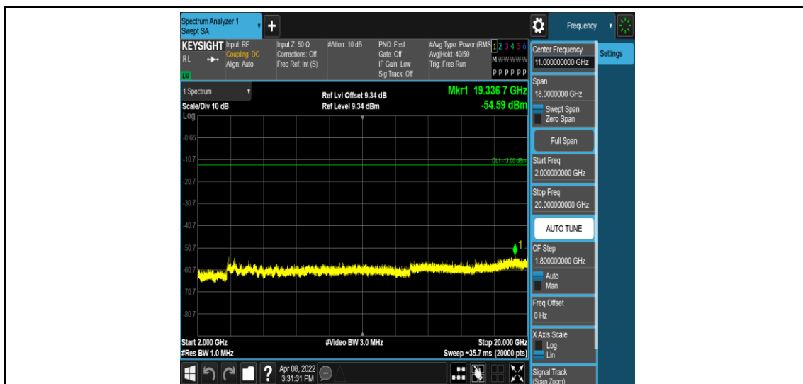
Band2-10MHz-QPSK-18650-1RB#0-Range5:2000~20000MHz
