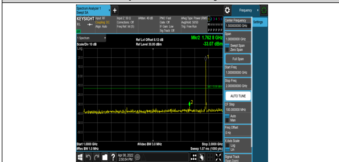
Band2-3MHz-16QAM-18900-1RB#0-Range4:1000~2000MHz
