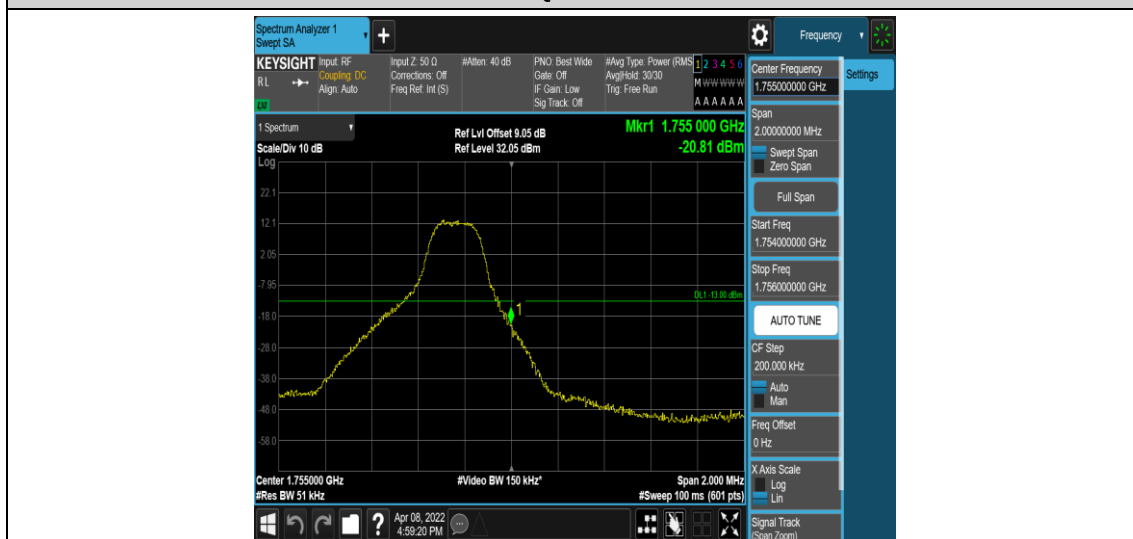
Band4-3MHz-QPSK-20385-1RB#14
