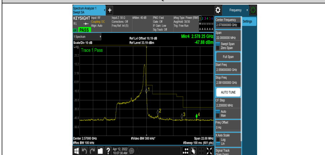
Band7-5MHz-16QAM-21425-1RB#24
