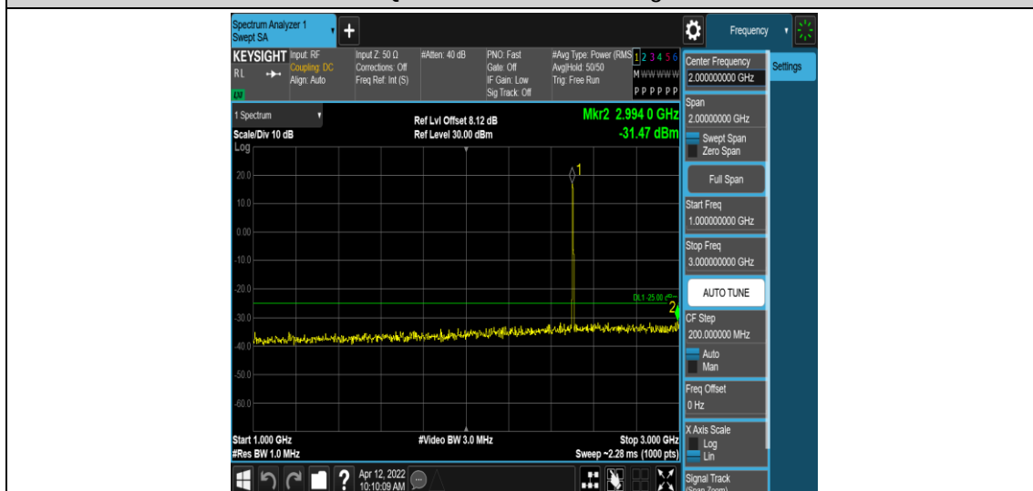
Band7-5MHz-16QAM-20775-1RB#0-Range4:1000~3000MHz
