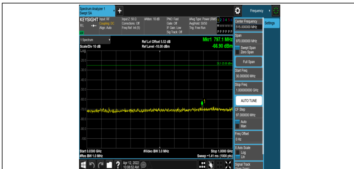
Band7-5MHz-QPSK-20775-1RB#0-Range3:30~1000MHz
