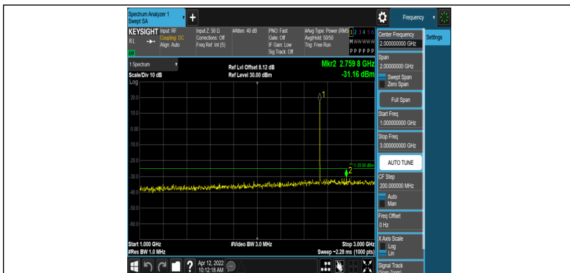
Band7-5MHz-16QAM-21100-1RB#0-Range4:1000~3000MHz
