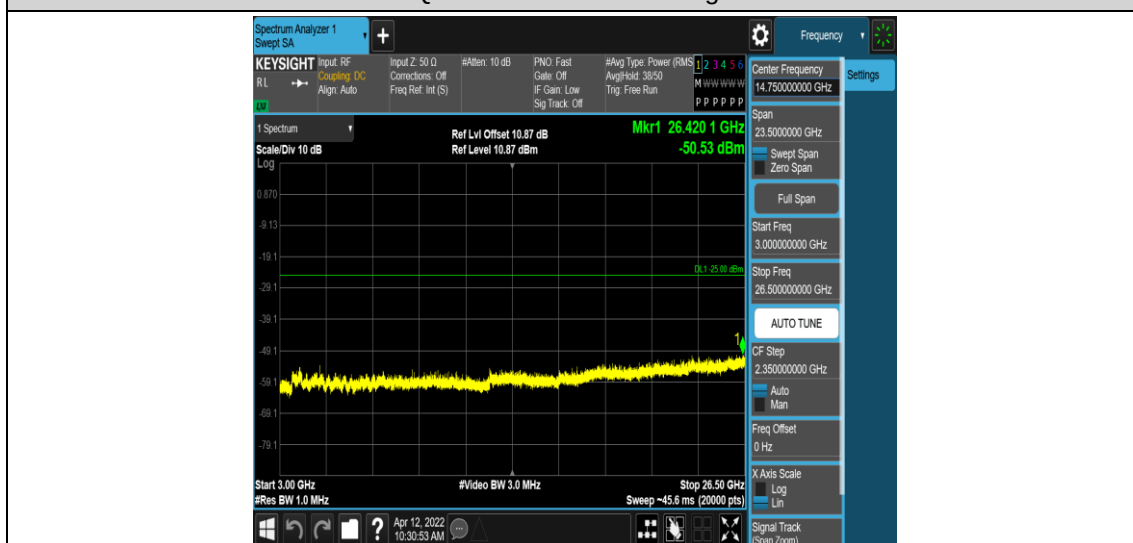
Band7-10MHz-16QAM-20800-1RB#0-Range5:3000~26500MHz
