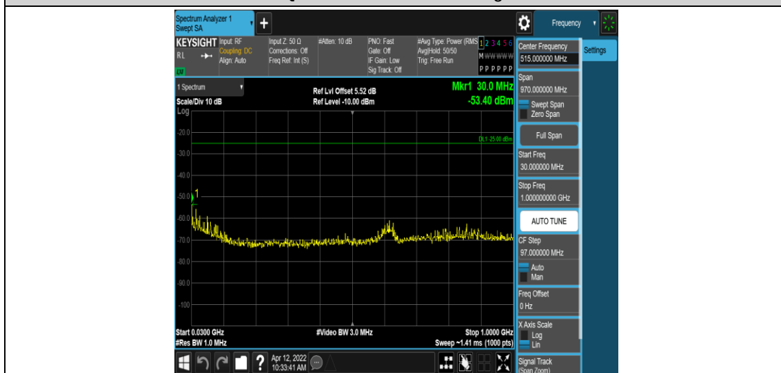
Band7-10MHz-QPSK-21400-1RB#0-Range3:30~1000MHz
