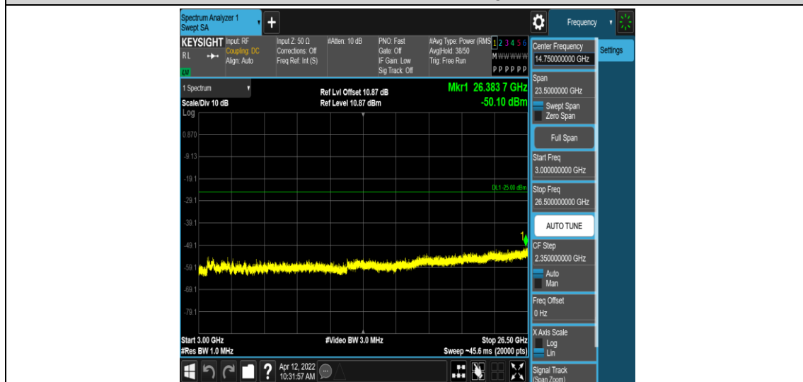
Band7-10MHz-QPSK-21100-1RB#0-Range5:3000~26500MHz
