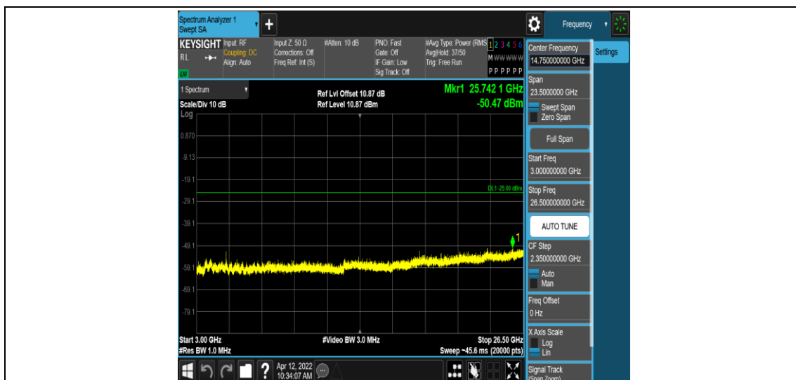
Band7-10MHz-QPSK-21400-1RB#0-Range5:3000~26500MHz
