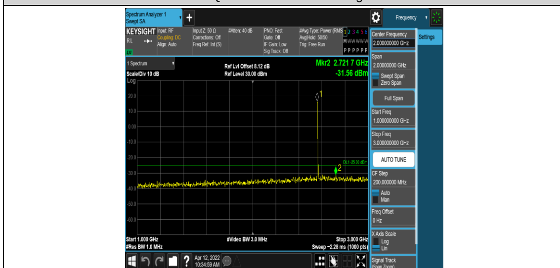
Band7-10MHz-16QAM-21400-1RB#0-Range4:1000~3000MHz
