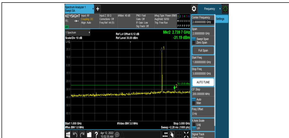
Band7-15MHz-QPSK-21100-1RB#0-Range4:1000~3000MHz
