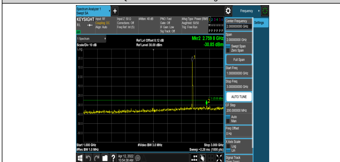
Band7-15MHz-QPSK-21375-1RB#0-Range4:1000~3000MHz
