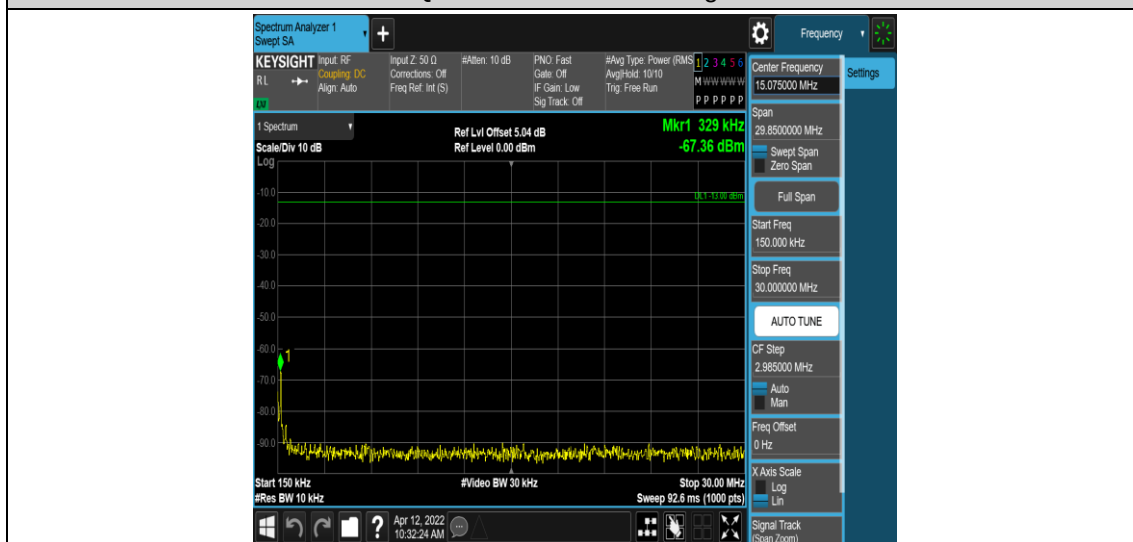
Band7-10MHz-16QAM-21100-1RB#0-Range2:0.15~30MHz
