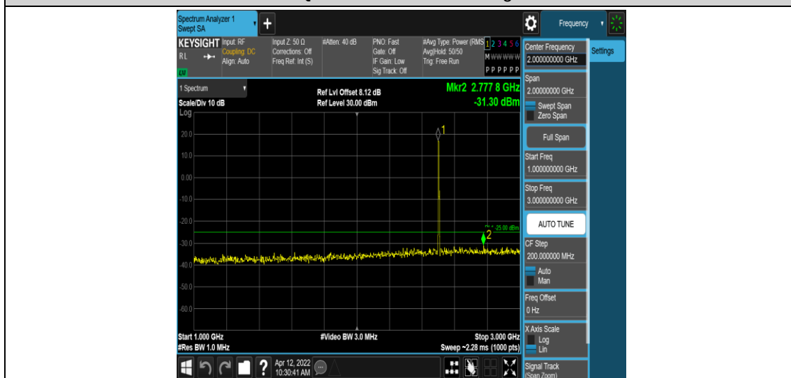
Band7-10MHz-16QAM-20800-1RB#0-Range4:1000~3000MHz
