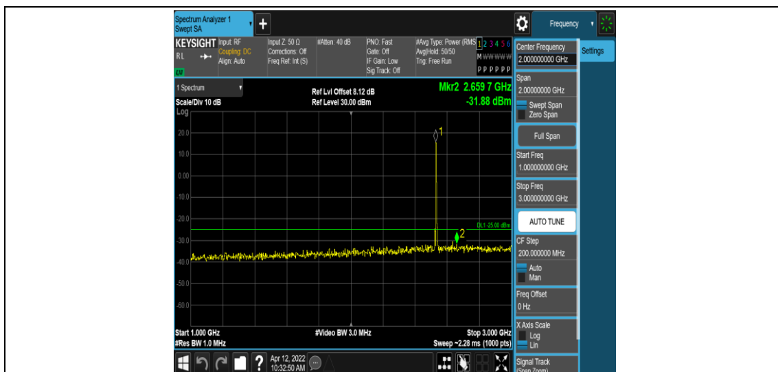
Band7-10MHz-16QAM-21100-1RB#0-Range4:1000~3000MHz
