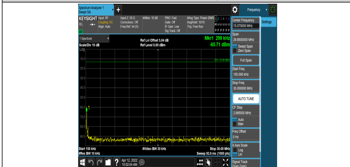
Band7-15MHz-QPSK-21100-1RB#0-Range2:0.15~30MHz
