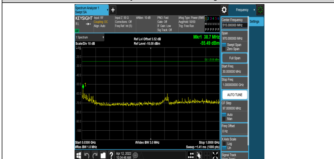
Band7-10MHz-16QAM-21400-1RB#0-Range3:30~1000MHz
