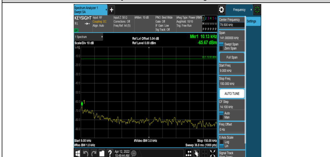
Band7-15MHz-QPSK-20825-1RB#0-Range1:0.009~0.15MHz
