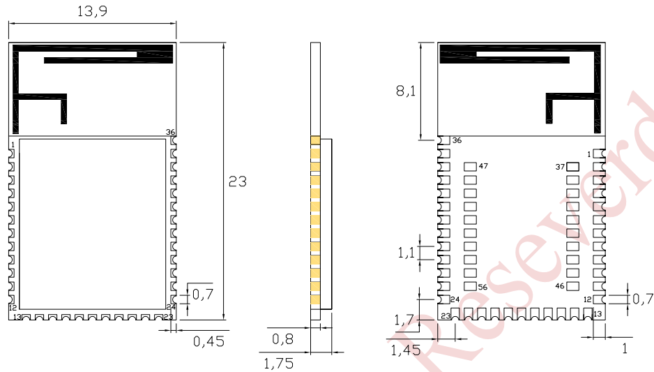
Figure 5.1 Dimensions of BB840F(top view)
