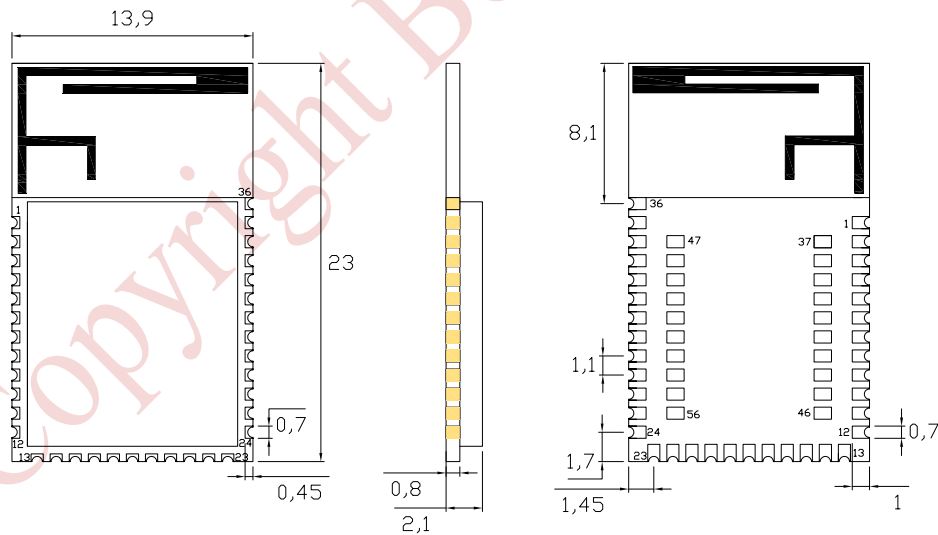
Figure 5.2 Dimensions of BB840FS(top view)
