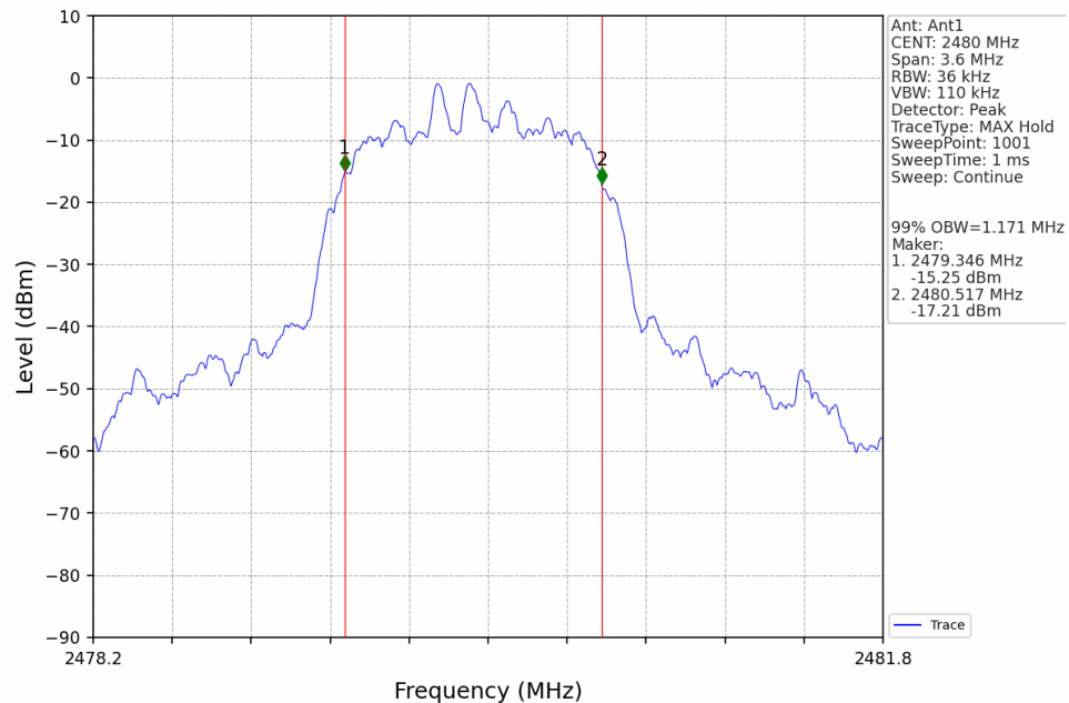
Pi/4DQPSK_2DH5_HCH_2480MHz_Ant1_NTNV
