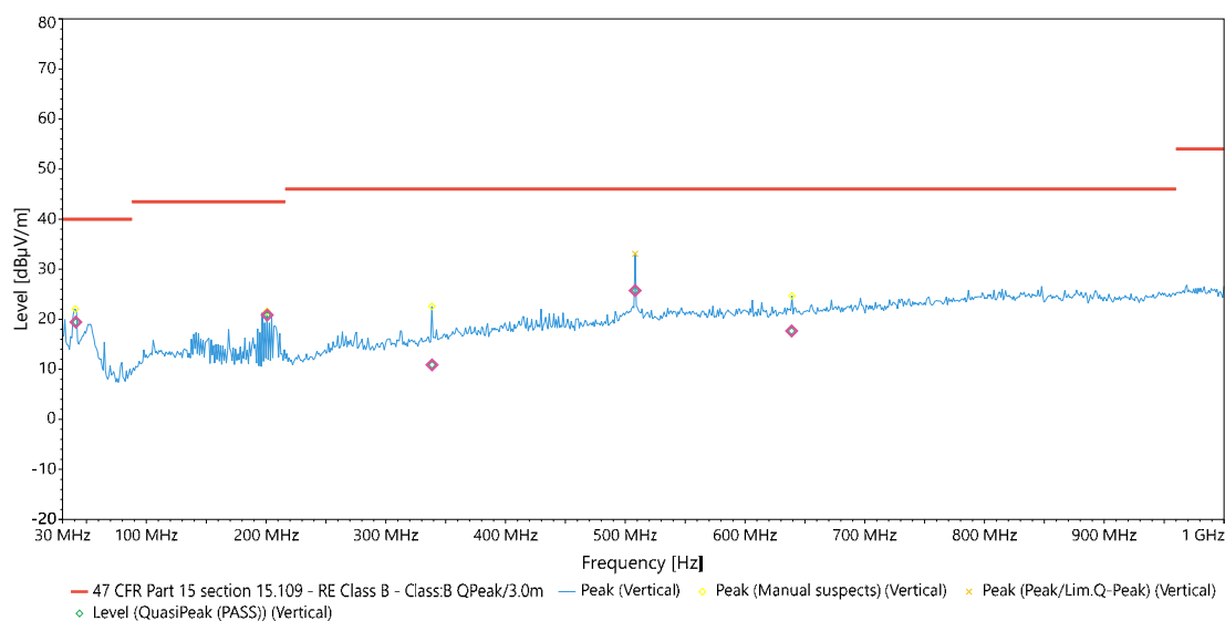
#1 - 30MHz-1GHz (Vertical)
