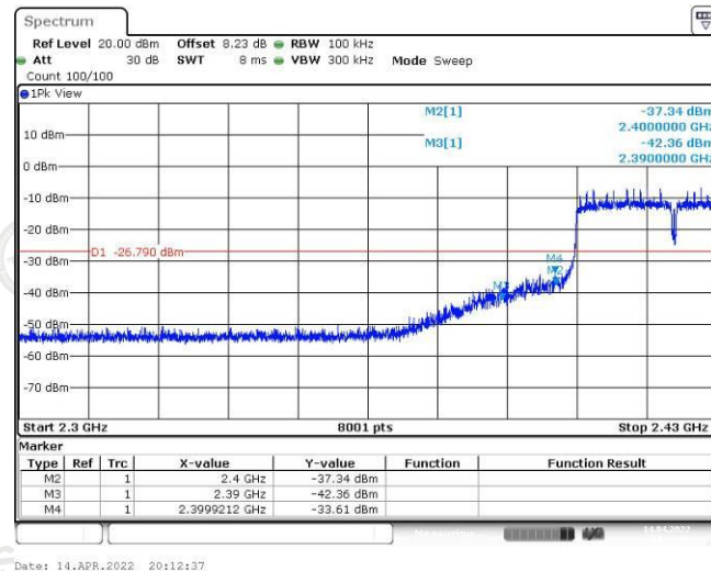
Left bandedge
