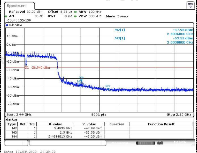
Right bandedge
