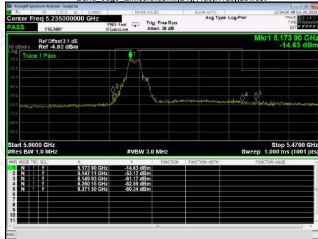
Band edge Emission,UNII(B1),11ac(HT20),Lowest
