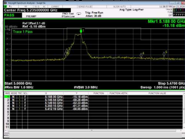
Band edge Emission,UNII(B1),11,Lowest
