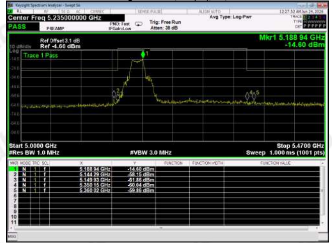
Band edge Emission,UNII(B1),11n,Lowest
