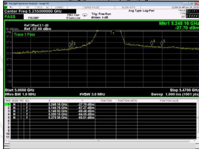
Band edge Emission,UNII(B1),11a,Highest
