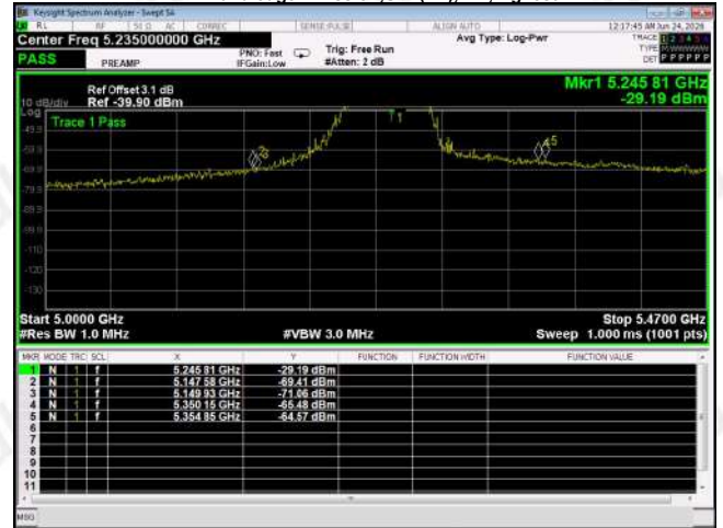
Band edge Emission,UNII(B1),11n,Highest
