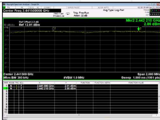
8-DPSK
