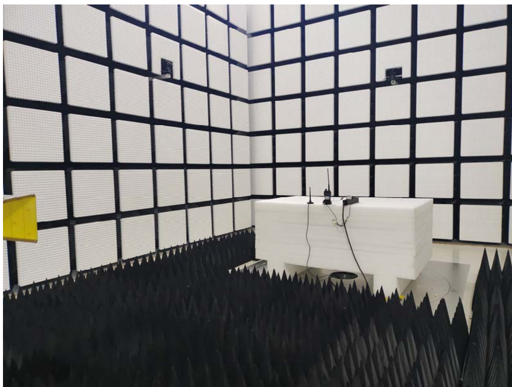
Radiated Emission Above 1GHz Rear View M3/M4
