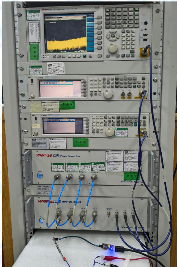
Photo of Setup for Conducted Measurement
