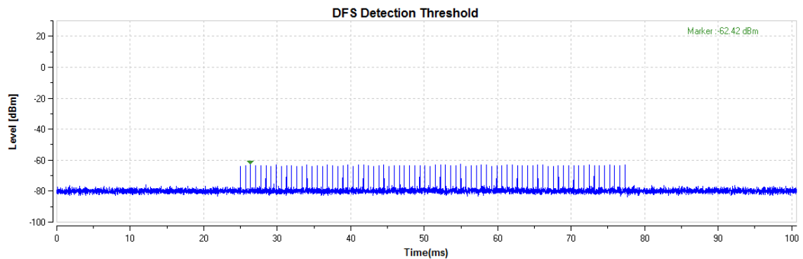
Radar Singal 1
