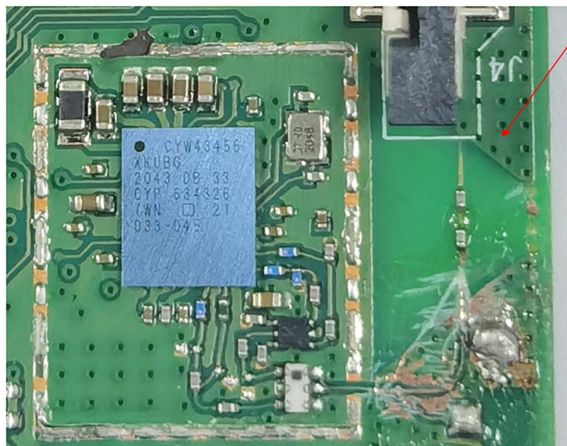
PCB Antenna
