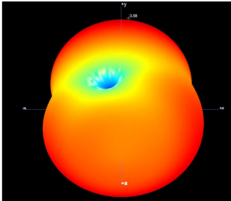
B1.2 3D Pattern for 433MHz
