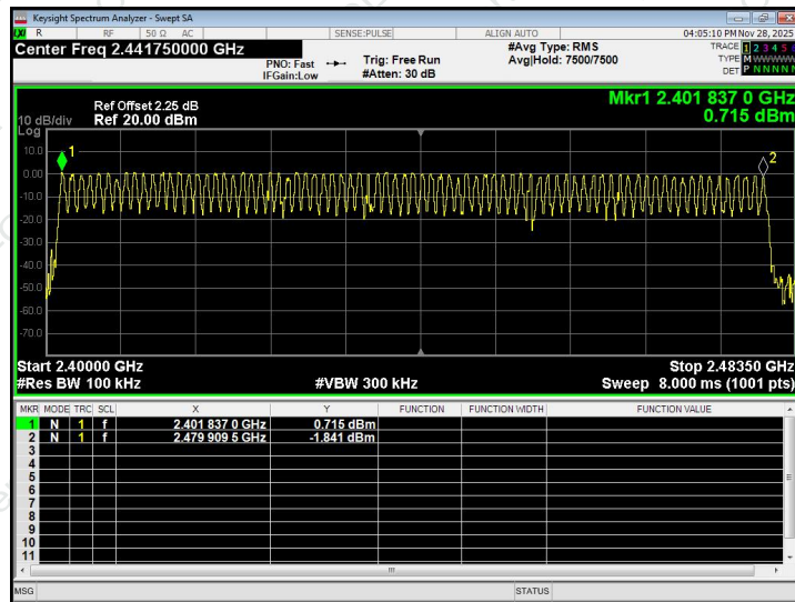
GFSK - 1-DH1 Test Plots
