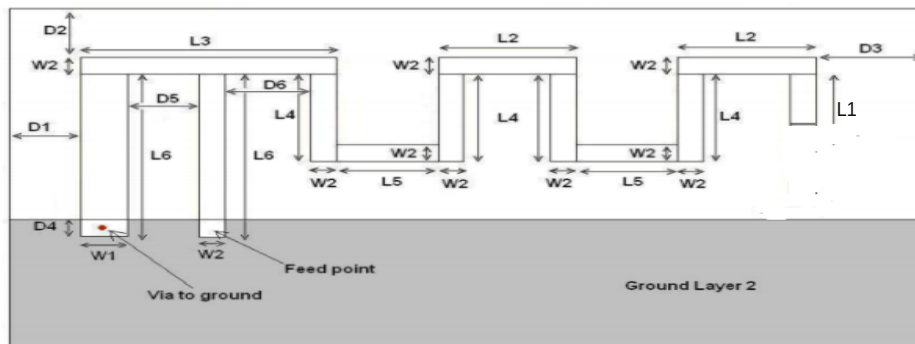
Figure 3: Antenna Dimensions
