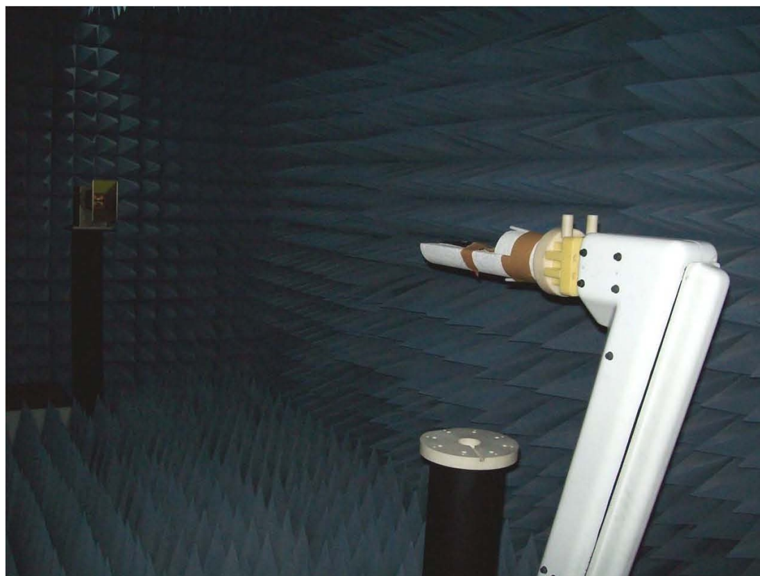
The Environment of Antenna Radiation Pattern
