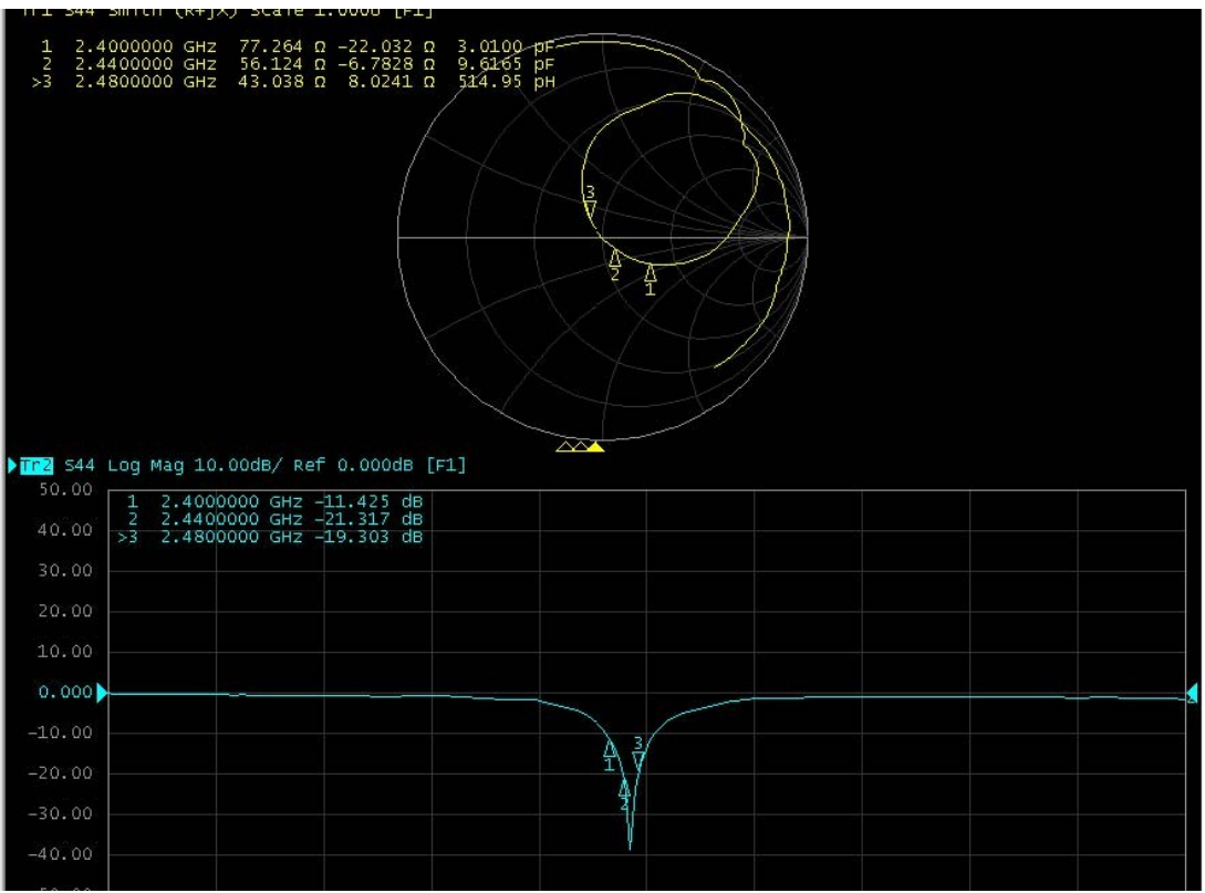
Return Loss
