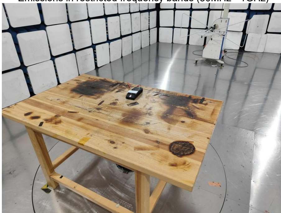
Emissions in restricted frequency bands (30MHz - 1GHz)
