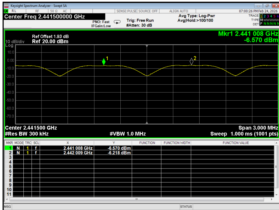
Carrier_Frequencies_Separation_(Hopping)_NVNT_ANT1_2-DH1_Hopping
