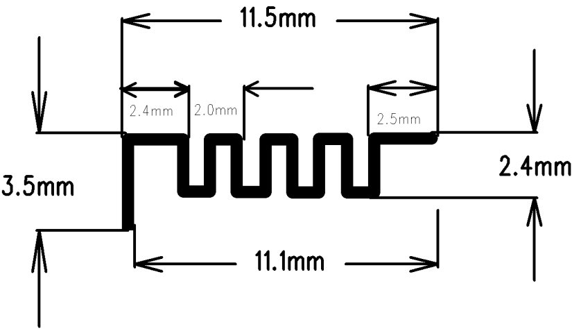
Antenna Photo & Length (mm)
