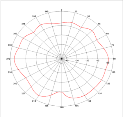
Far-field Power Distribution(H+V) on Y-Z Plane
