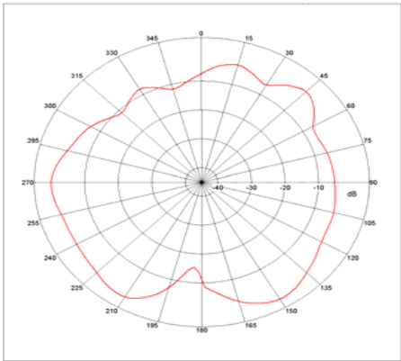
Far-field Power Distribution(H+V) on X-Z Plane
