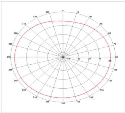
Far-field Power Distribution(H+V) on X-Y Plane
