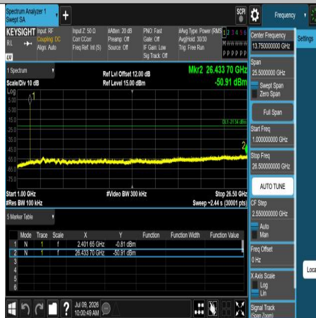
BLE_2M-Ant1-2402-1000~26500-PASS
