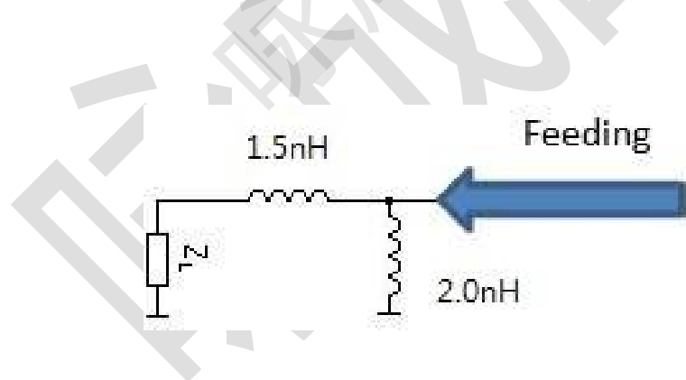
Suggested Matching Circuit
