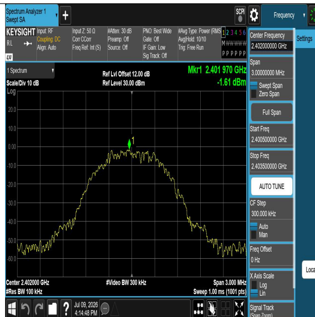
BLE_1M-Ant1-2402-0~Reference-PASS
