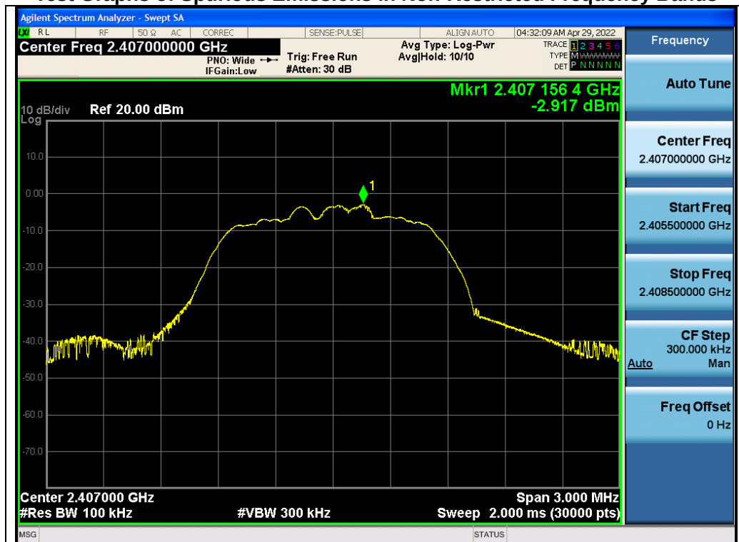
Test_Graph_GFSK_ANT1_2407_Reference Level
