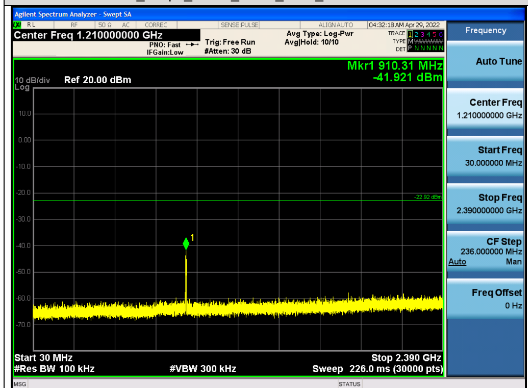
Test_Graph_GFSK_ANT1_2407_Lower Band Emissions
