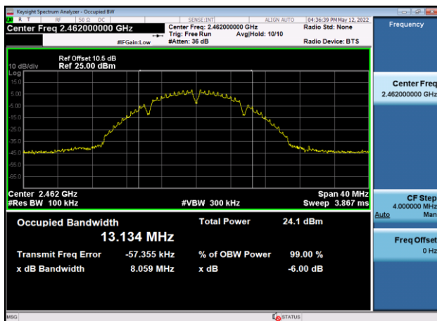
6dB Bandwidth-802.11b,2462MHz,Ant9
