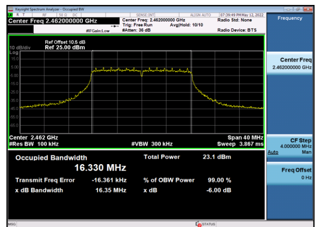
6dB Bandwidth-802.11g,2462MHz,Ant7
