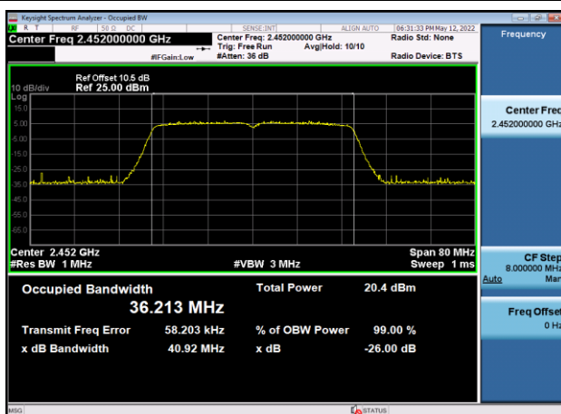
99% Bandwidth-802.11n(HT40),2452MHz ,Ant9
