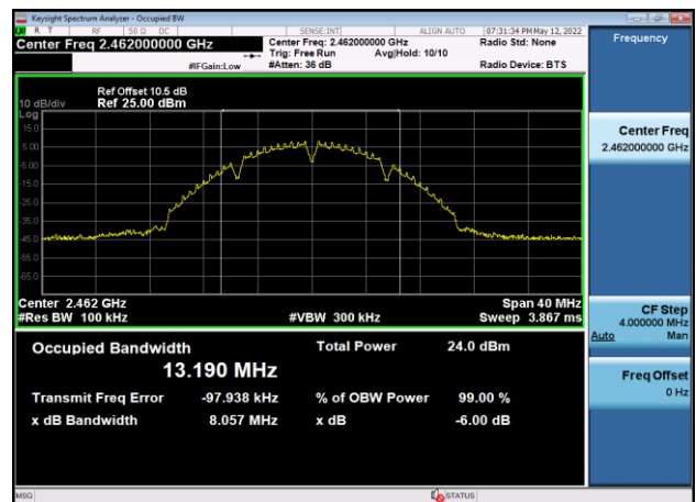
6dB Bandwidth-802.11b,2462MHz,Ant7
