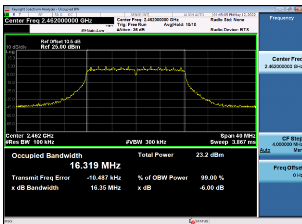
6dB Bandwidth-802.11g,2462MHz,Ant9
