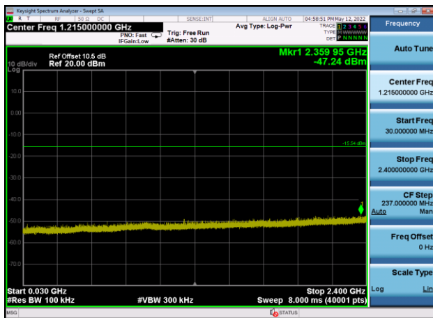
,Plot 3,30MHz~2400MHz-802.11g,2462MHz ,Ant9
