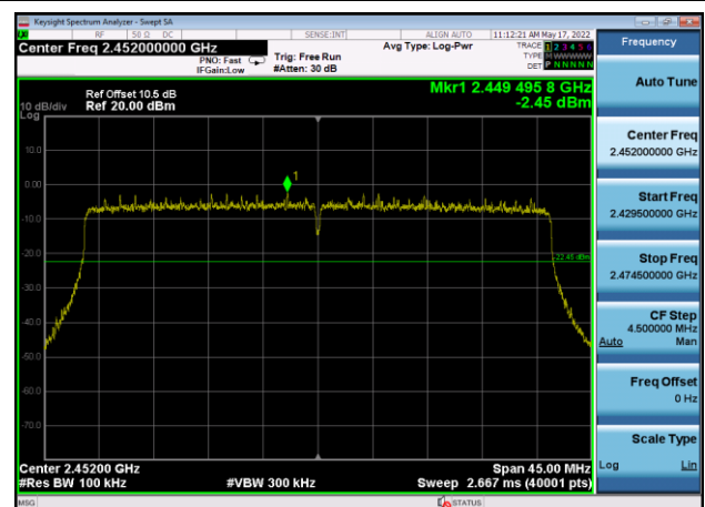
,Plot 1,Reference Level-802.11ax(HT40 ) ,2452MHz,Ant7
