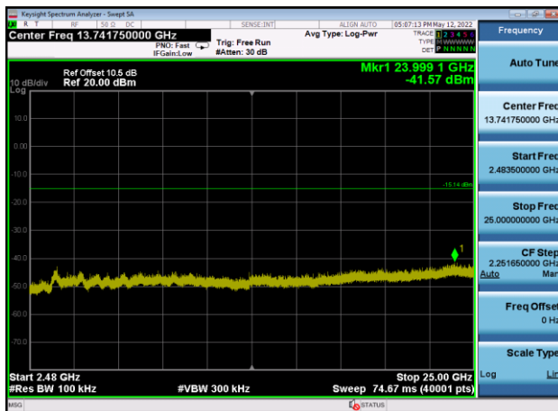
,Plot 4,2483.5MHz~25000MHz-802.11g ,2437MHz,Ant9
