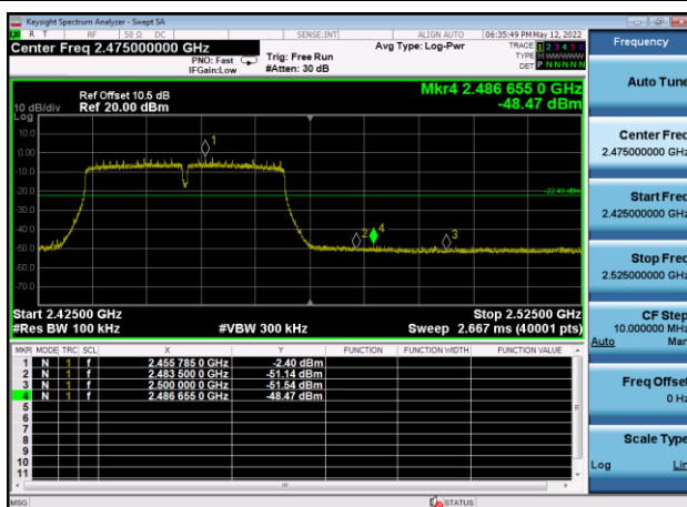
,Plot 2,Band Edge-802.11n(HT40) ,2452MHz,Ant9
