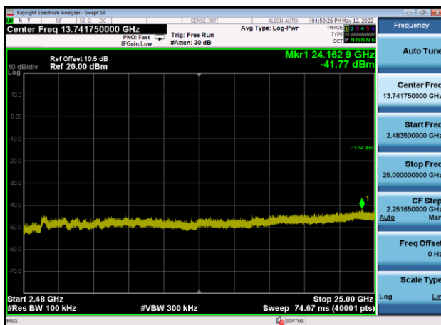
,Plot 4,2483.5MHz~25000MHz-802.11g ,2462MHz,Ant9
