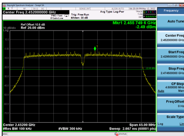
,Plot 1,Reference Level-802.11n(HT40) ,2452MHz,Ant9
