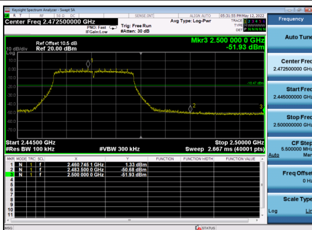
,Plot 2,Band Edge-802.11n(HT20) ,2462MHz,Ant9
