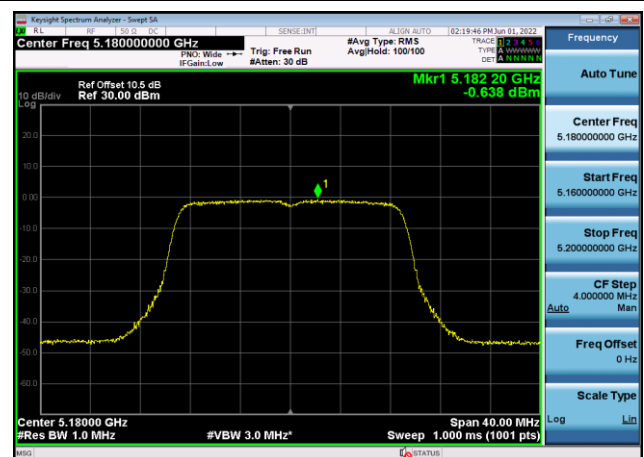
U-NII-1 Power spectral density-802.11 ac(20MHz),5180MHz,Ant8
