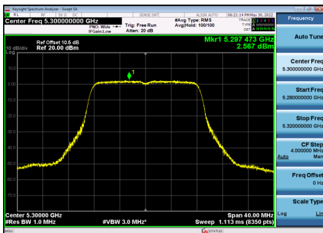
U-NII-2a Power spectral density-802.1 1a(20MHz),5300MHz,Ant9
