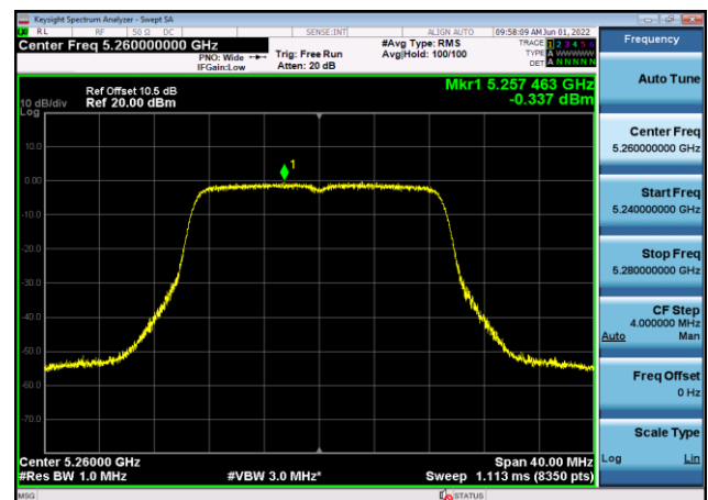
U-NII-2a Power spectral density-802.1 1ac(20MHz),5260MHz,Ant8
