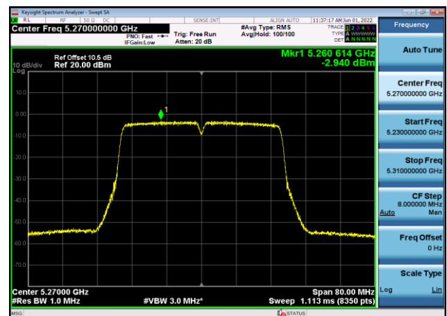
U-NII-2a Power spectral density-802.1 1n(40MHz),5270MHz,Ant8
