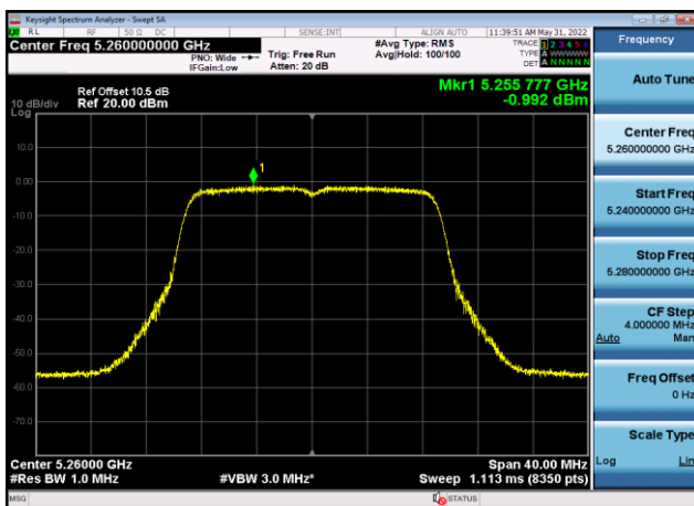
U-NII-2a Power spectral density-802.1 1n(20MHz),5260MHz,Ant9
