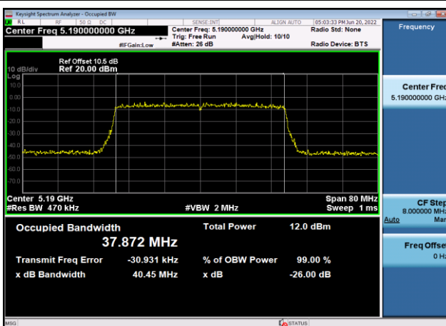
U-NII-1 99% Bandwidth-802.11ax(40MHz) ,5190MHz,Ant9
