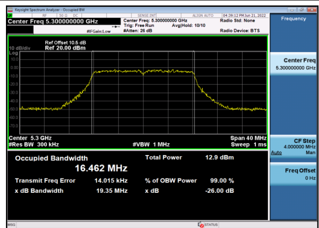
U-NII-2a 99% Bandwidth-802.11a(20MHz) ,5300MHz,Ant8
