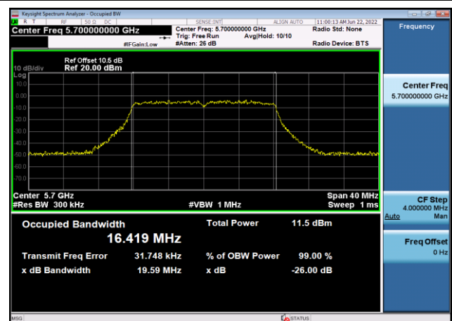
U-NII-2c 99% Bandwidth-802.11a(20MHz) ,5700MHz,Ant8
