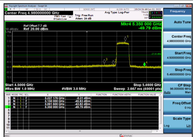
U-NII-1 ,Plot 1,Band Edge-802.11ax(80 MHz),5210MHz,Ant8
