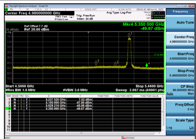
U-NII-1 ,Plot 1,Band Edge-802.11a(20M Hz),5240MHz,Ant8
