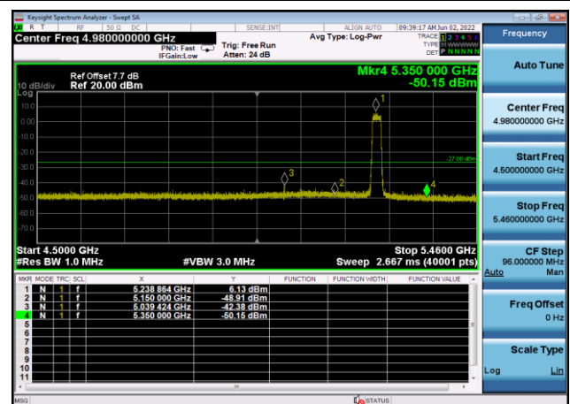
U-NII-1 ,Plot 1,Band Edge-802.11ax(20 MHz),5240MHz,Ant8
