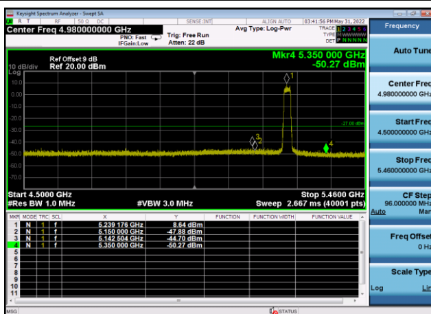
U-NII-1 ,Plot 1,Band Edge-802.11ax(20 MHz),5240MHz,Ant9
