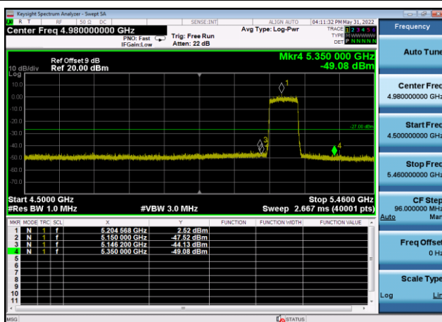
U-NII-1 ,Plot 1,Band Edge-802.11ax(80 MHz),5210MHz,Ant9
