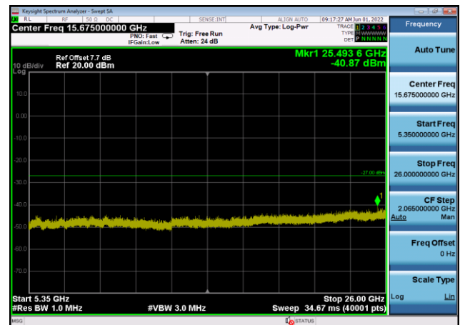
U-NII-1 ,Plot 3,5350MHz~26000MHz-802. 11a(20MHz),5240MHz,Ant8
