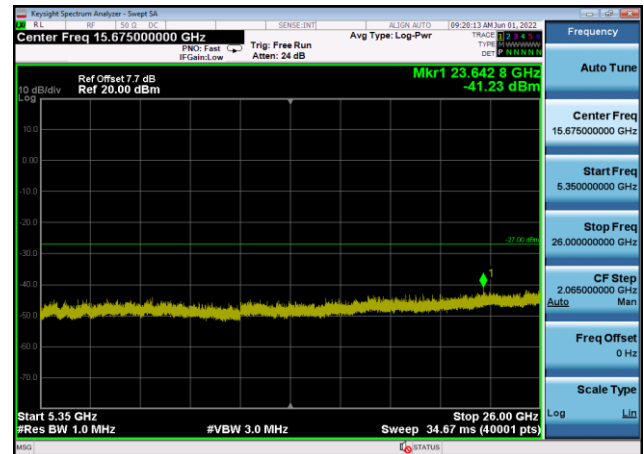
U-NII-1 ,Plot 3,5350MHz~26000MHz-802. 11a(20MHz),5220MHz,Ant8
