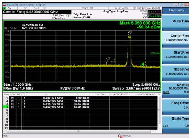
U-NII-2a ,Plot 1,Band Edge-802.11n(20 MHz),5300MHz,Ant9
