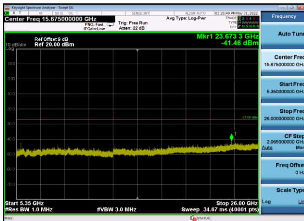
U-NII-1 ,Plot 3,5350MHz~26000MHz-802. 11a(20MHz),5240MHz,Ant9
