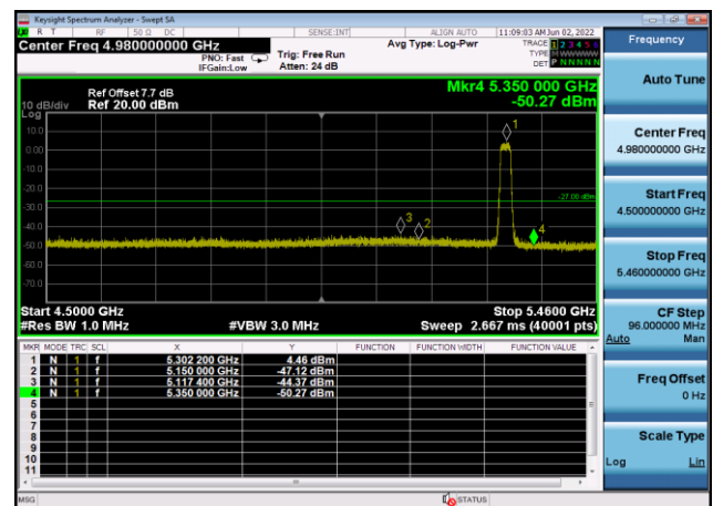
U-NII-2a ,Plot 1,Band Edge-802.11n(20 MHz),5320MHz,Ant8
