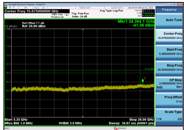
U-NII-1 ,Plot 3,5350MHz~26000MHz-802. 11ax(20MHz),5240MHz,Ant8
