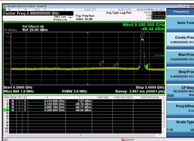
U-NII-2a ,Plot 1,Band Edge-802.11n(20 MHz),5320MHz,Ant9
