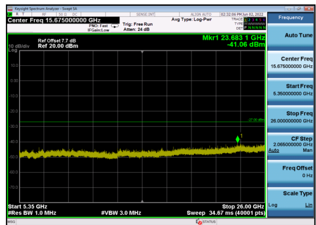
U-NII-2a ,Plot 3,5350MHz~26000MHz-802 .11ax(160MHz),5250MHz,Ant8
