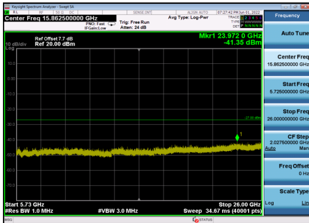
U-NII-2c ,Plot 3,5725MHz~26000MHz-802 .11ax(80MHz),5610MHz,Ant8
