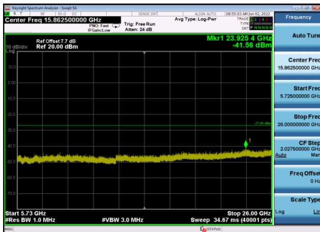
U-NII-2c ,Plot 3,5725MHz~26000MHz-802 .11ax(20MHz),5700MHz,Ant8
