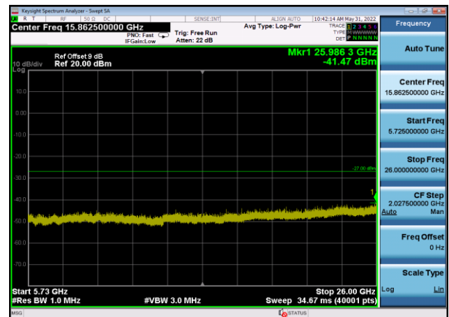
U-NII-2c ,Plot 3,5725MHz~26000MHz-802 .11ax(40MHz),5510MHz,Ant9
