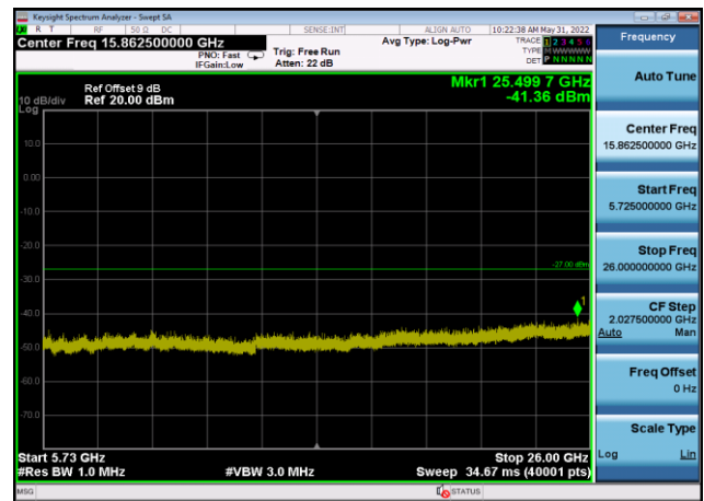
U-NII-2c ,Plot 3,5725MHz~26000MHz-802 .11ax(20MHz),5500MHz,Ant9
