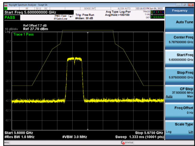
U-NII-3 ,Plot 1,Band Edge-802.11n(40M Hz),5795MHz,Ant8
