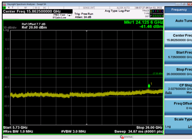
U-NII-2c ,Plot 3,5725MHz~26000MHz-802 .11ax(20MHz),5600MHz,Ant8
