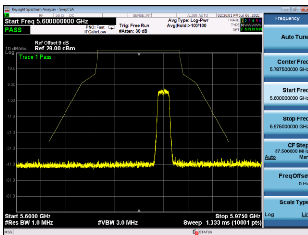
U-NII-3 ,Plot 1,Band Edge-802.11n(20M Hz),5825MHz,Ant9
