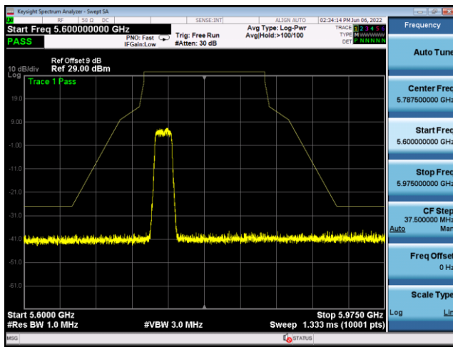
U-NII-3 ,Plot 1,Band Edge-802.11n(20M Hz),5785MHz,Ant9
