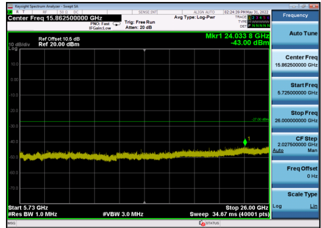
U-NII-2c ,Plot 3,5725MHz~26000MHz-802 .11ax(20MHz),5500MHz,Ant9
