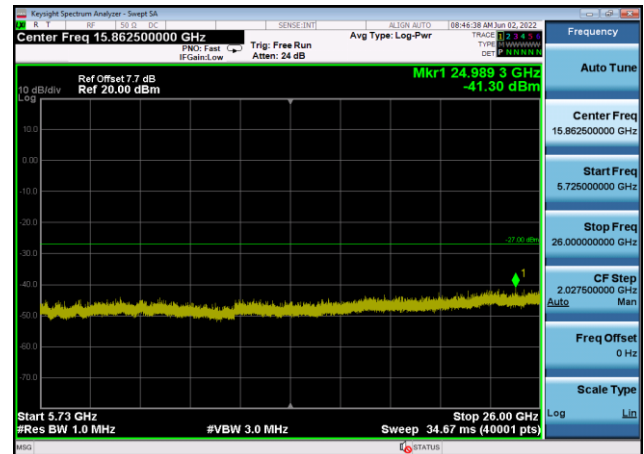
U-NII-2c ,Plot 3,5725MHz~26000MHz-802 .11a(20MHz),5700MHz,Ant8
