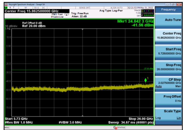
U-NII-2c ,Plot 3,5725MHz~26000MHz-802 .11ax(80MHz),5530MHz,Ant9
