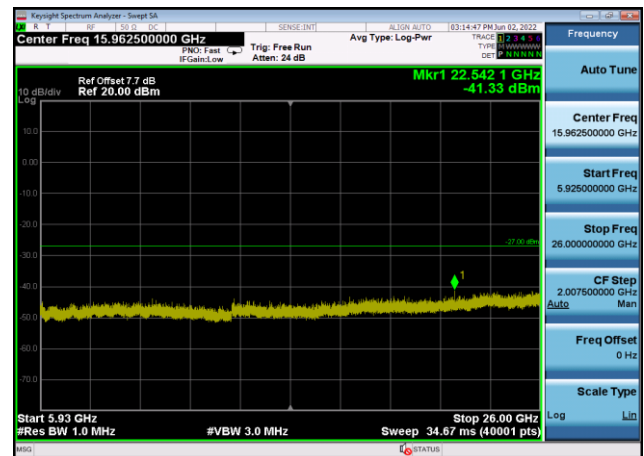
U-NII-3 ,Plot 3,5925MHz~26000MHz-802.11n(40MHz),5795MHz,Ant8
