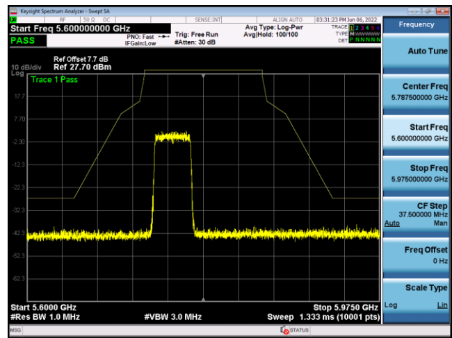
U-NII-3 ,Plot 1,Band Edge-802.11ax(40 MHz),5795MHz,Ant8
