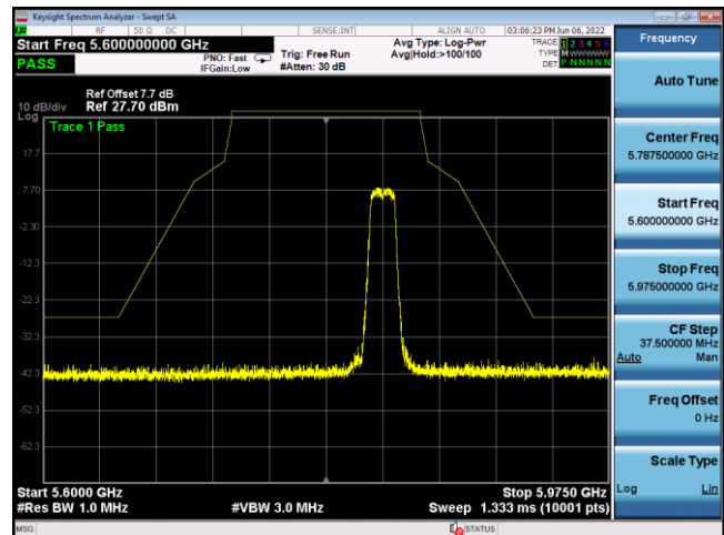
U-NII-3 ,Plot 1,Band Edge-802.11a(20 Hz),5825MHz,Ant8
