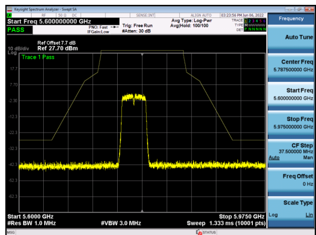
U-NII-3 ,Plot 1,Band Edge-802.11ac(80 MHz),5775MHz,Ant8
