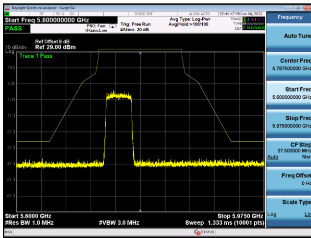
U-NII-3 ,Plot 1,Band Edge-802.11ax(40 MHz),5795MHz,Ant9
