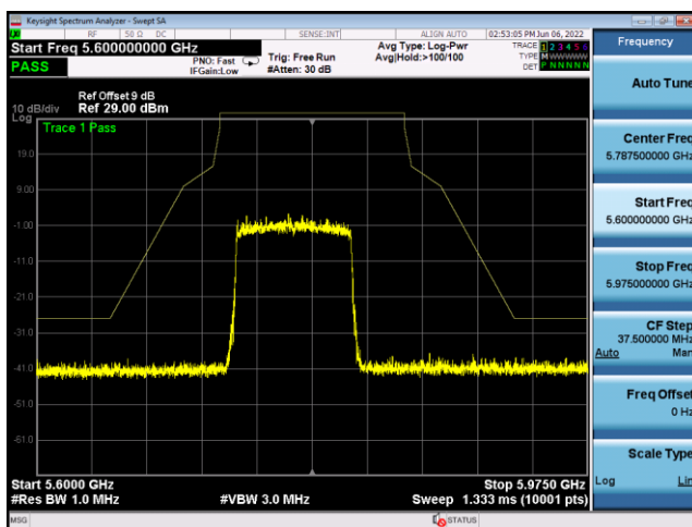
U-NII-3 ,Plot 1,Band Edge-802.11ax(80 MHz),5775MHz,Ant9
