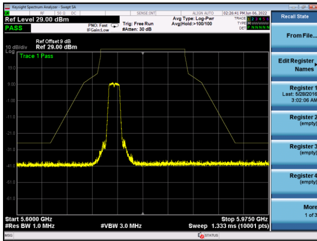
U-NII-3 ,Plot 1,Band Edge-802.11a(20 Hz),5785MHz,Ant9
