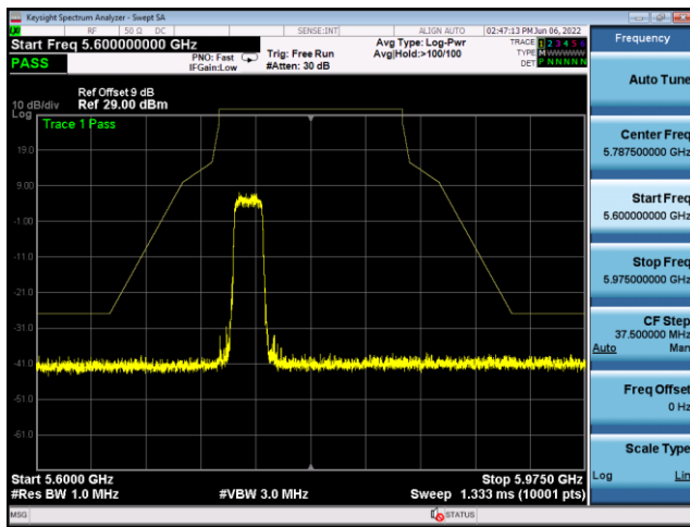
U-NII-3 ,Plot 1,Band Edge-802.11ax(20 MHz),5785MHz,Ant9
