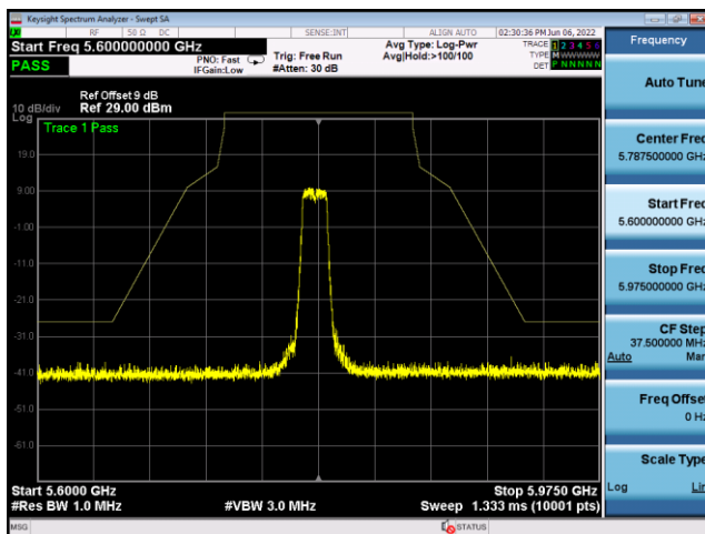
U-NII-3 ,Plot 1,Band Edge-802.11a(20 Hz),5825MHz,Ant9
