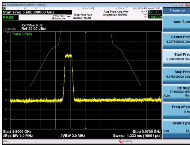
U-NII-3 ,Plot 1,Band Edge-802.11ac(20 MHz),5785MHz,Ant9
