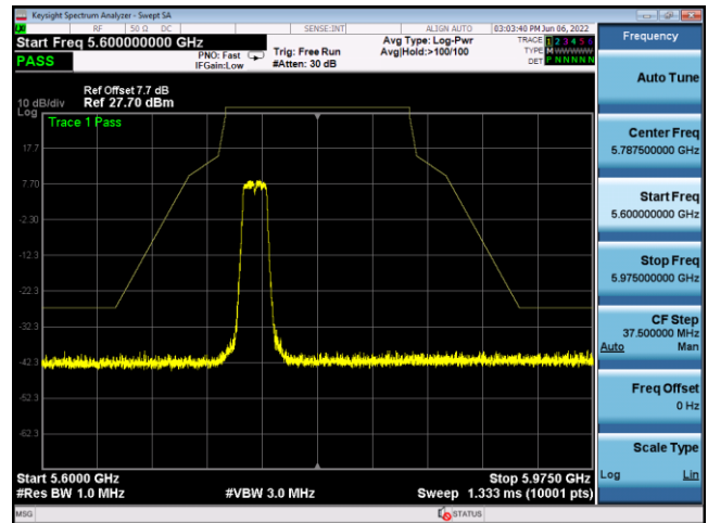
U-NII-3 ,Plot 1,Band Edge-802.11a(20 Hz),5785MHz,Ant8
