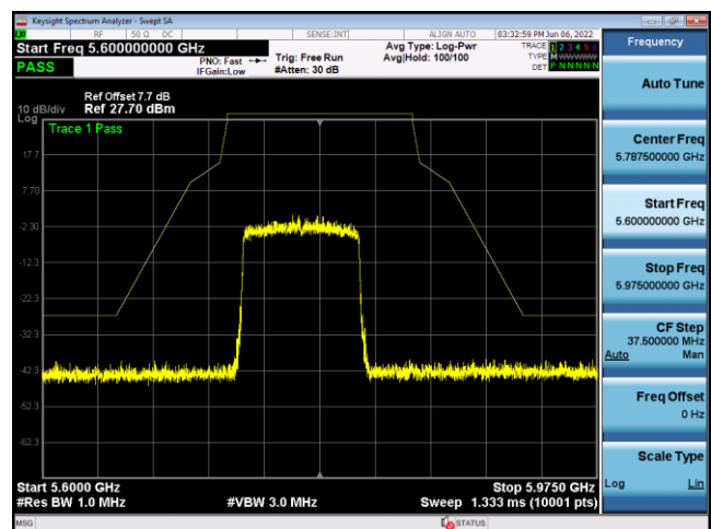
U-NII-3 ,Plot 1,Band Edge-802.11ax(80 MHz),5775MHz,Ant8
