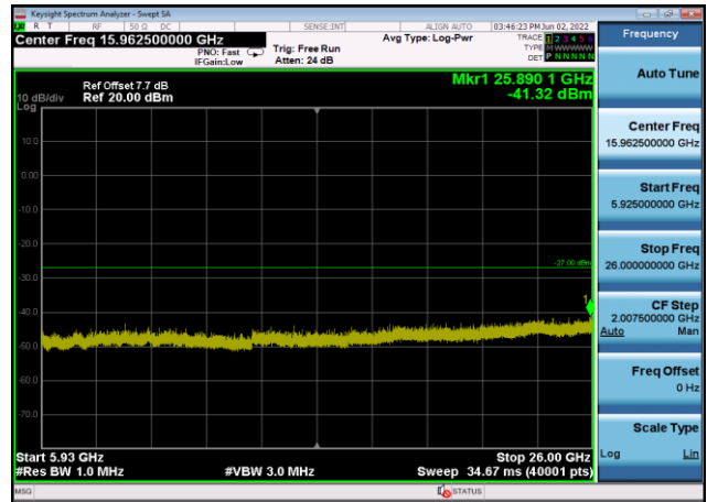
U-NII-3 ,Plot 3,5925MHz~26000MHz-802. 11ax(20MHz),5825MHz,Ant8
