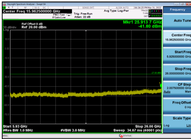
U-NII-3 ,Plot 3,5925MHz~26000MHz-802. 11ax(20MHz),5785MHz,Ant9
