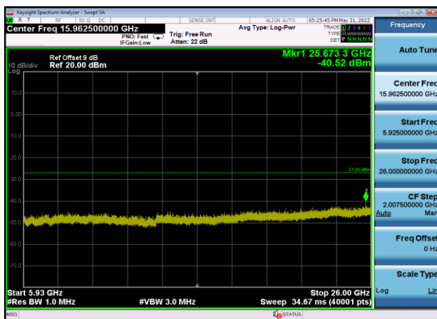
U-NII-3 ,Plot 3,5925MHz~26000MHz-802. 11a(20MHz),5825MHz,Ant9
