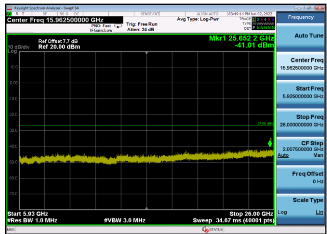
U-NII-3 ,Plot 3,5925MHz~26000MHz-802. 11ax(20MHz),5825MHz,Ant8
