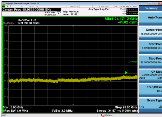
U-NII-3 ,Plot 3,5925MHz~26000MHz-802. 11a(20MHz),5785MHz,Ant9
