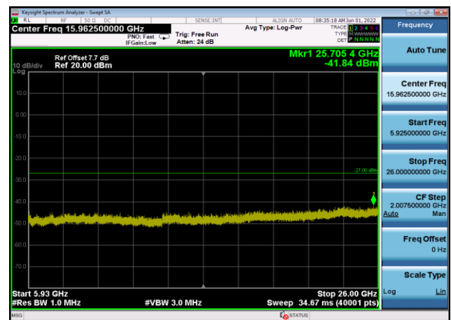
U-NII-3 ,Plot 3,5925MHz~26000MHz-802. 11a(20MHz),5825MHz,Ant8
