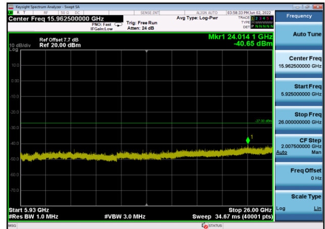
U-NII-3 ,Plot 3,5925MHz~26000MHz-802. 11ax(40MHz),5795MHz,Ant8
