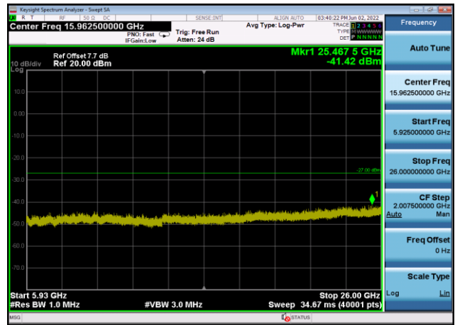
U-NII-3 ,Plot 3,5925MHz~26000MHz-802. 11ax(20MHz),5785MHz,Ant8
