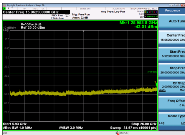
U-NII-3 ,Plot 3,5925MHz~26000MHz-802. 11ax(80MHz),5775MHz,Ant9
