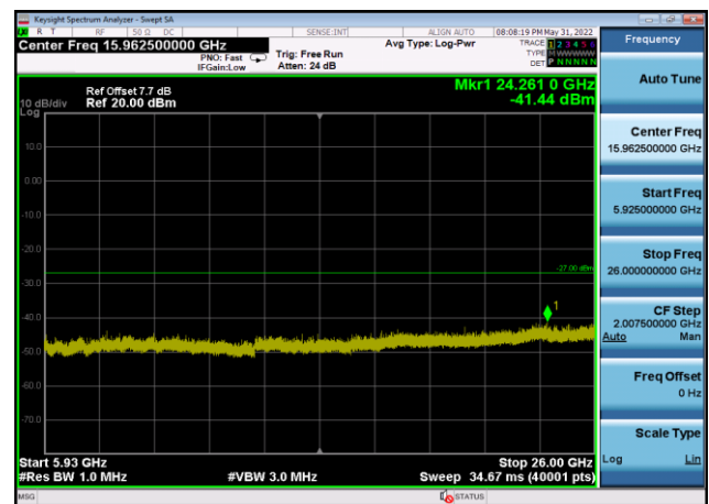
U-NII-3 ,Plot 3,5925MHz~26000MHz-802. 11ax(80MHz),5775MHz,Ant8
