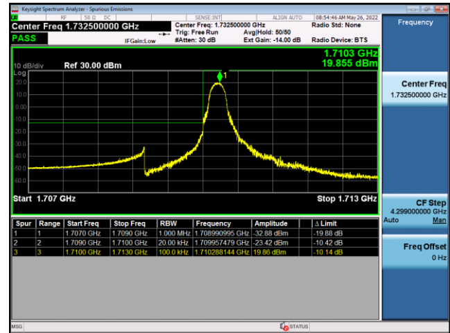
FDD4-1.4MHz-16QAM-LCH-6RB#0
