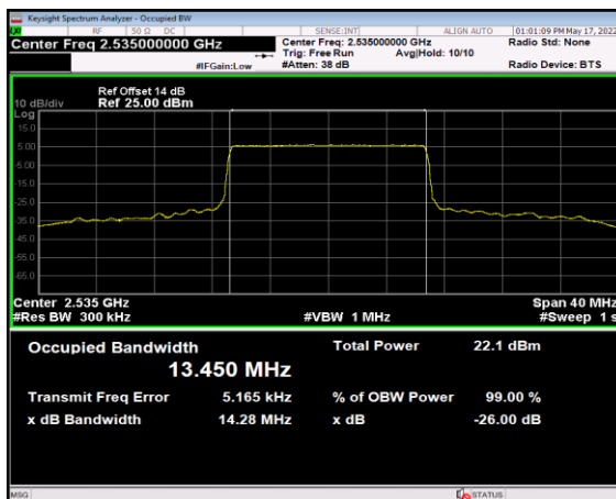
FDD07_MidRange_20_2535_QPSK
