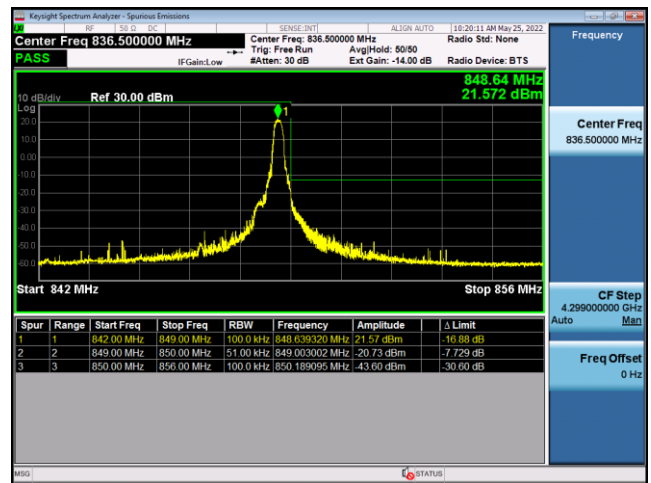
FDD5-5MHz-16QAM-HCH-25RB#0
