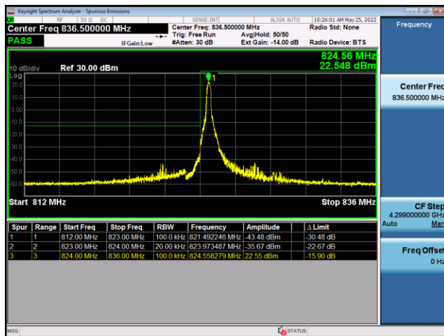
FDD5-10MHz-QPSK-LCH-50RB#0
