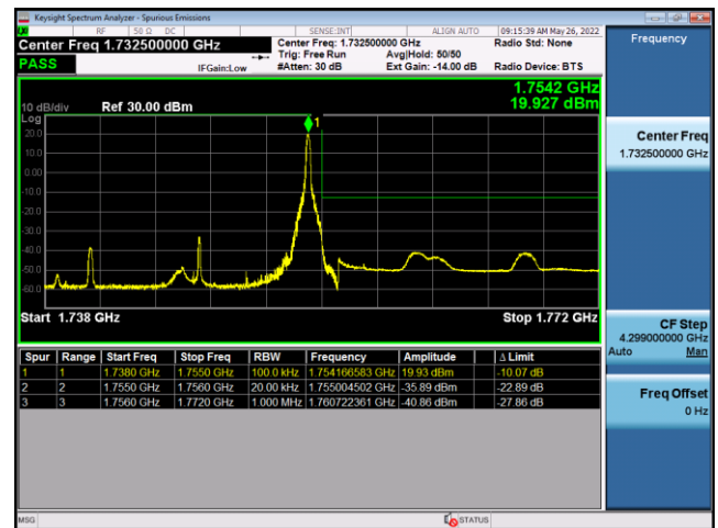
FDD4-15MHz-16QAM-HCH-75RB#0
