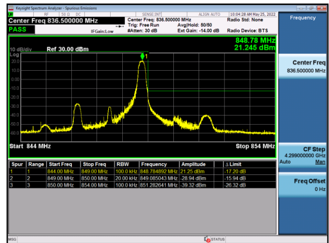
FDD5-3MHz-16QAM-HCH-15RB#0
