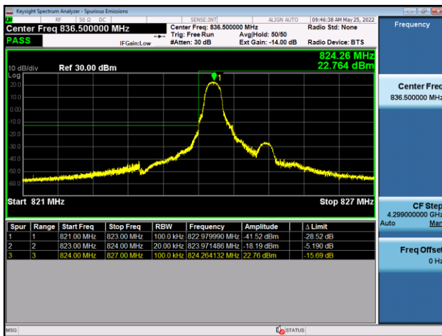
FDD5-1.4MHz-QPSK-LCH-6RB#0
