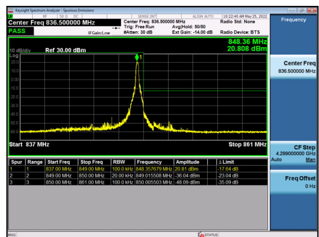
FDD5-10MHz-16QAM-HCH-1RB#49
