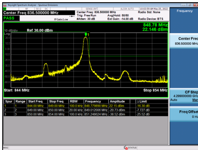
FDD5-3MHz-QPSK-HCH-15RB#0
