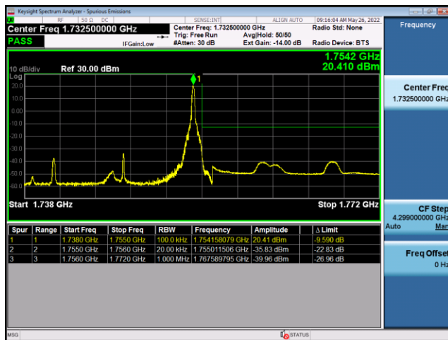
FDD4-15MHz-QPSK-HCH-75RB#0
