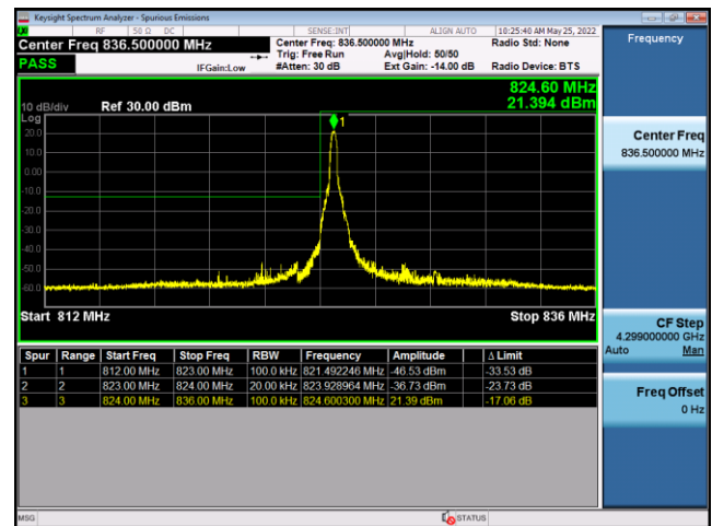
FDD5-10MHz-16QAM-LCH-50RB#0
