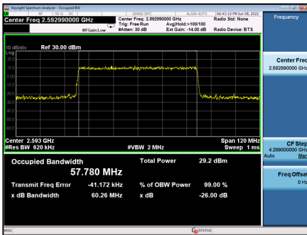
N41(60M)_CP-OFDM_256QAM_ Outer_Full_Mid_CH
