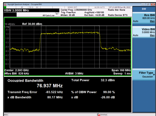
N41(80M)_DFT-s-OFDM_16QAM_ Outer_Full_Mid_CH
