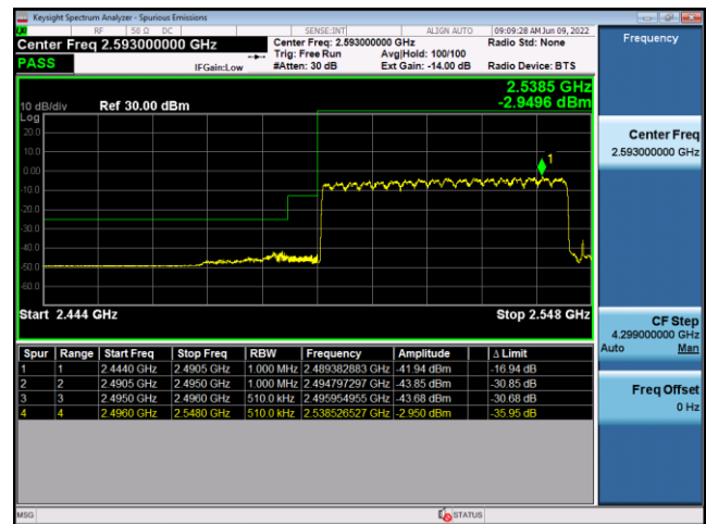
N41(50M)_CP-OFDM_QPSK_Edge_ Outer_Full_Low_CH
