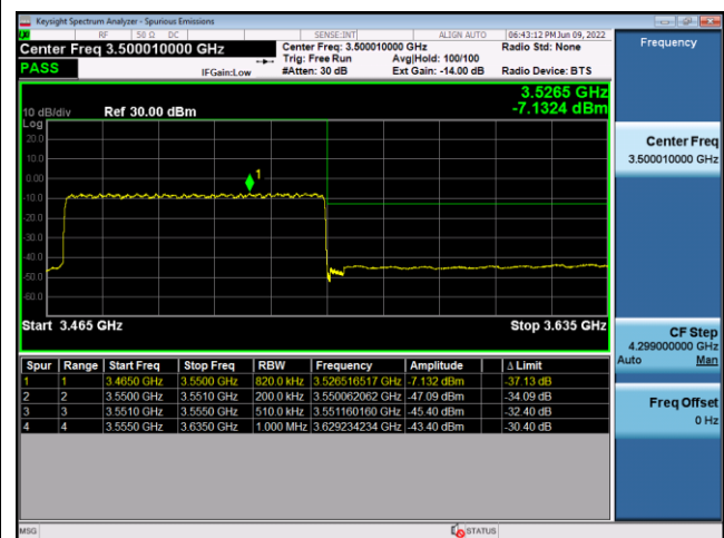
N77(80M)_CP-OFDM_QPSK_Edge_ Outer_Full_High_CH
