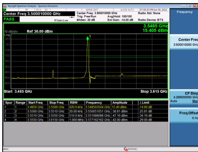
N77(60M)_CP-OFDM_QPSK_Edge_ 1RB_Right_High_CH
