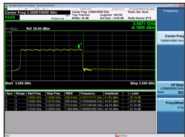
N77(40M)_CP-OFDM_QPSK_BPSK_Edge_ Outer_Full_High_CH
