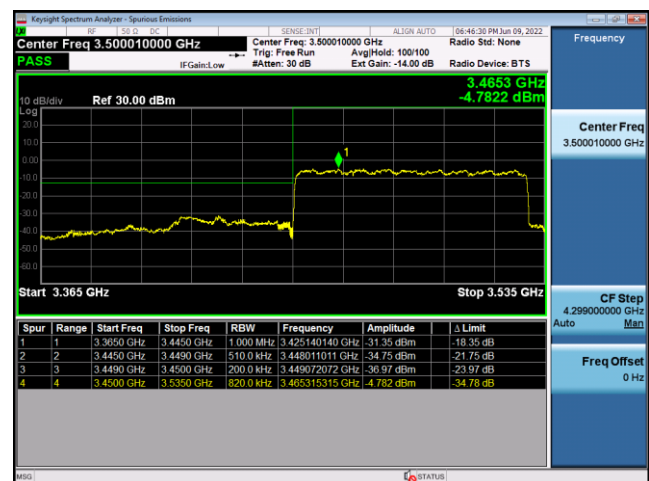
N77(80M)_DFT-s-OFDM_PI/2-BPSK_Edge_ Outer_Full_Low_CH
