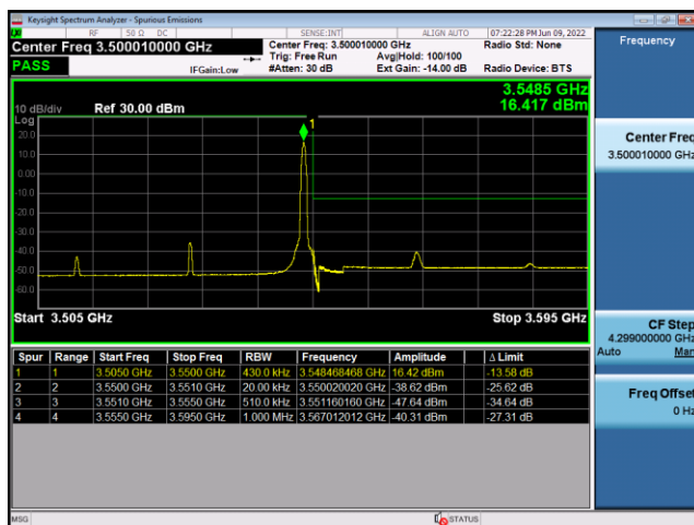
N77(40M)_CP-OFDM_QPSK_Edge_ 1RB_Left_High_CH
