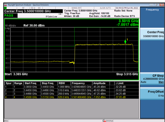
N77(60M)_CP-OFDM_QPSK_Edge_ Outer_Full_Low_CH
