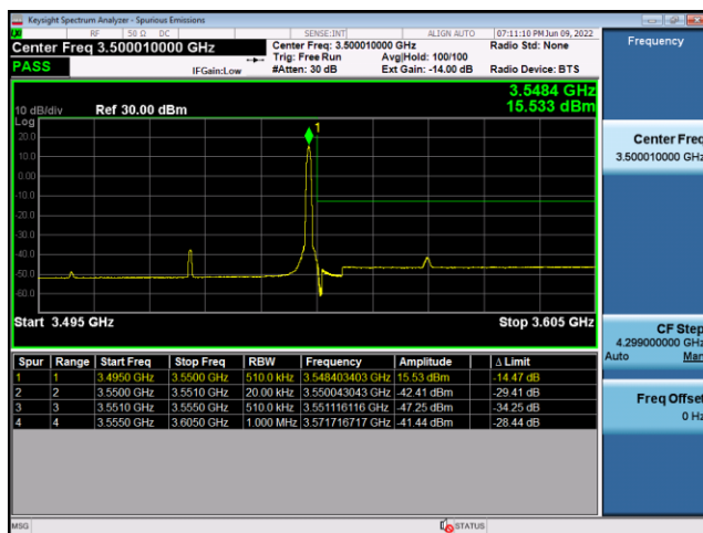
N77(50M)_DFT-s-OFDM_PI/2-BPSK_Edge_ 1RB_Right_High_CH
