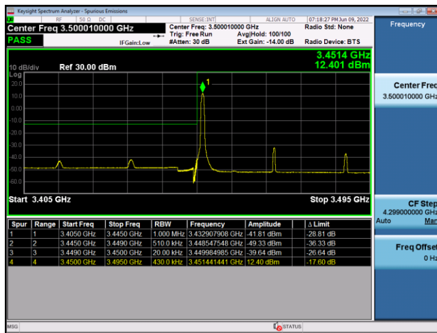
N77(40M)_DFT-s-OFDM_PI/2-BPSK_Edge_ 1RB_Right_High_CH
