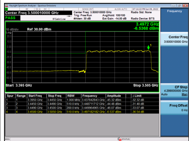
N77(50M)_DFT-s-OFDM_PI/2-BPSK_Edge_ Outer_Full_High_CH
