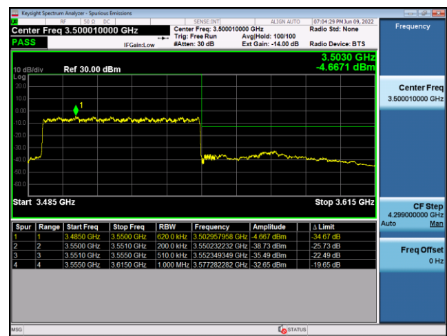
N77(60M)_CP-OFDM_QPSK_Edge_ Outer_Full_High_CH
