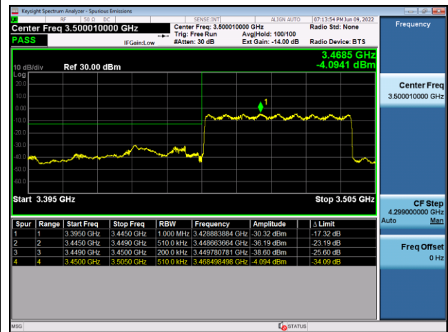
N77(50M)_CP-OFDM_QPSK_Edge_ Outer_Full_Low_CH
