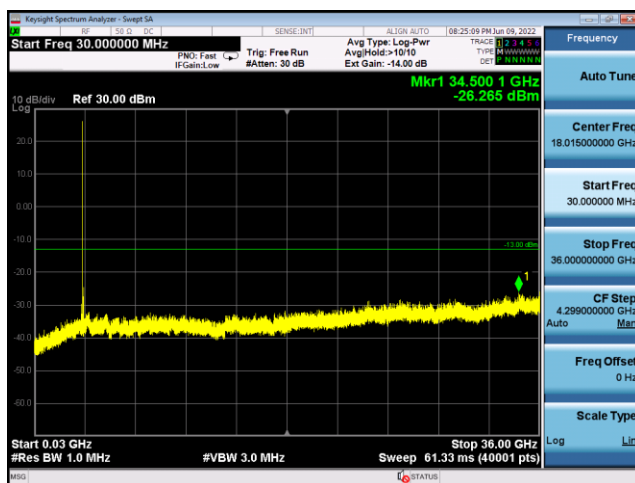
N77(90M)_DFT-s-OFDM_BPSK_ Edge_1RB_Left_High_CH
