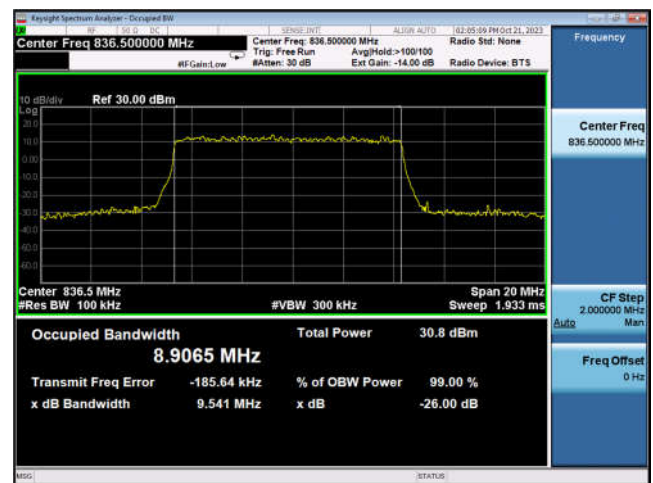
Band n5_10MHz_DFT-s-OFDM_16QAM_ Outer_Full_Mid_CH
