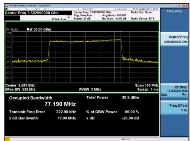
Band n41_80MHz_DFT-s-OFDM_16QAM_ Outer_Full_Mid_CH
