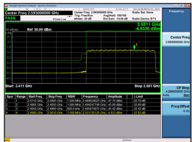
N41_80MHz_DFT-s-OFDM_PI/2-BPSK_Edge_ Outer_Full_Low_CH
