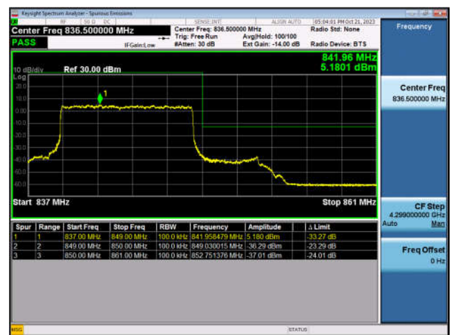
N5_15MHz_DFT-s-OFDM_PI/2-BPSK_Edge_ Outer_Full_Low_CH
