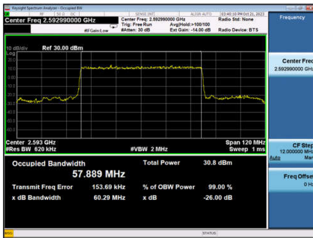
Band n41_60MHz_DFT-s-OFDM_QPSK_ Outer_Full_Mid_CH
