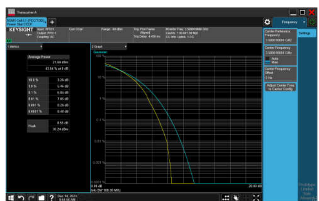
Band n77_100MHz_DFT-s-OFDM_256QAM_ Outer_Full_Mid_CH
