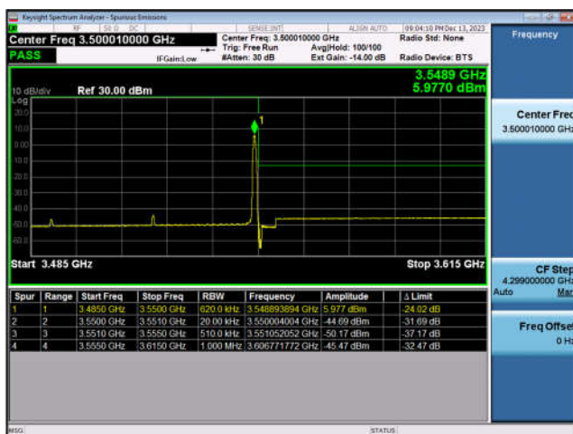
N77_60MHz_DFT-s-OFDM_PI/2-BPSK_Edge_ 1RB_Right_High_CH
