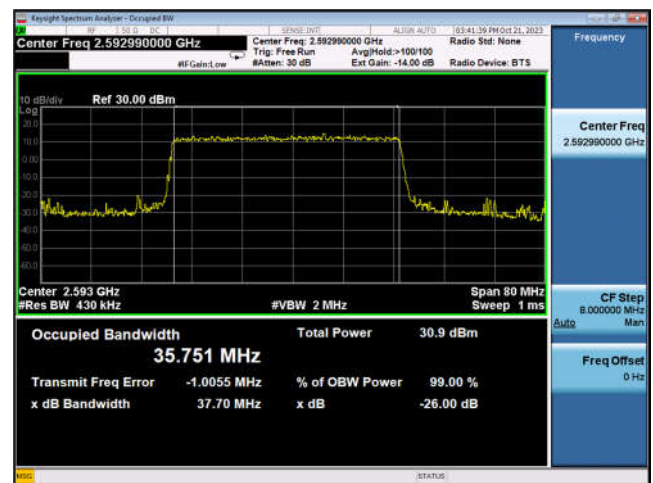
Band n41_40MHz_DFT-s-OFDM_16QAM_ Outer_Full_Mid_CH
