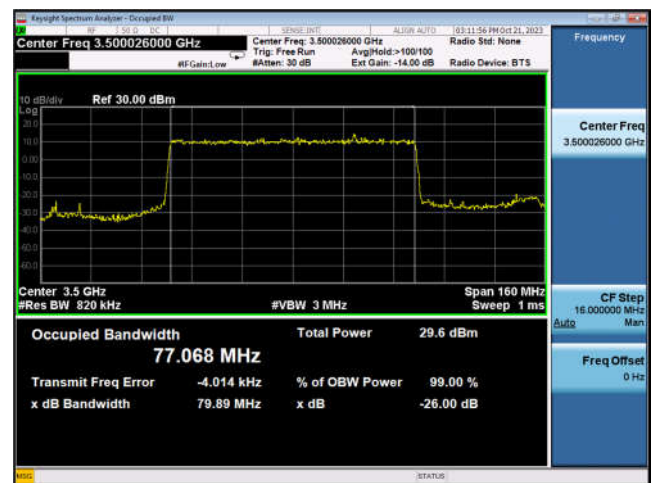
Band n78_80MHz_DFT-s-OFDM_QPSK_ Outer_Full_Mid_CH
