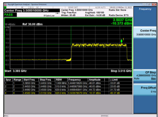
N77_60MHz_DFT-s-OFDM_PI/2-BPSK_Edge_ Outer_Full_High_CH
