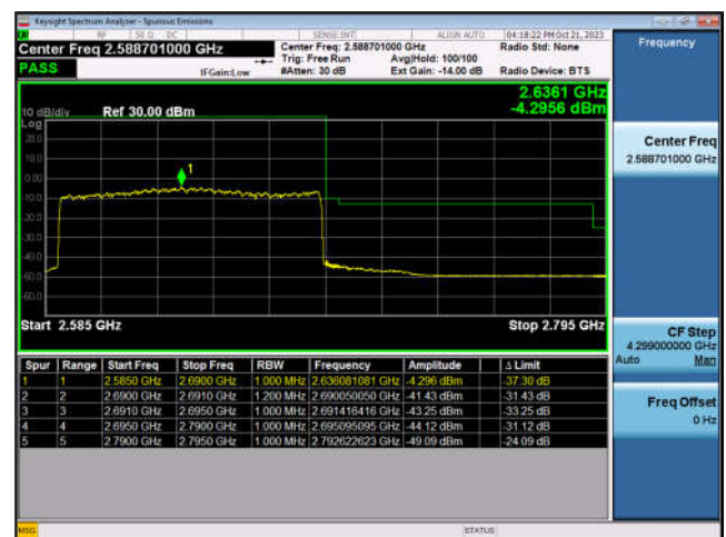
N41_100MHz_DFT-s-OFDM_PI/2-BPSK_Edge_ Outer_Full_High_CH
